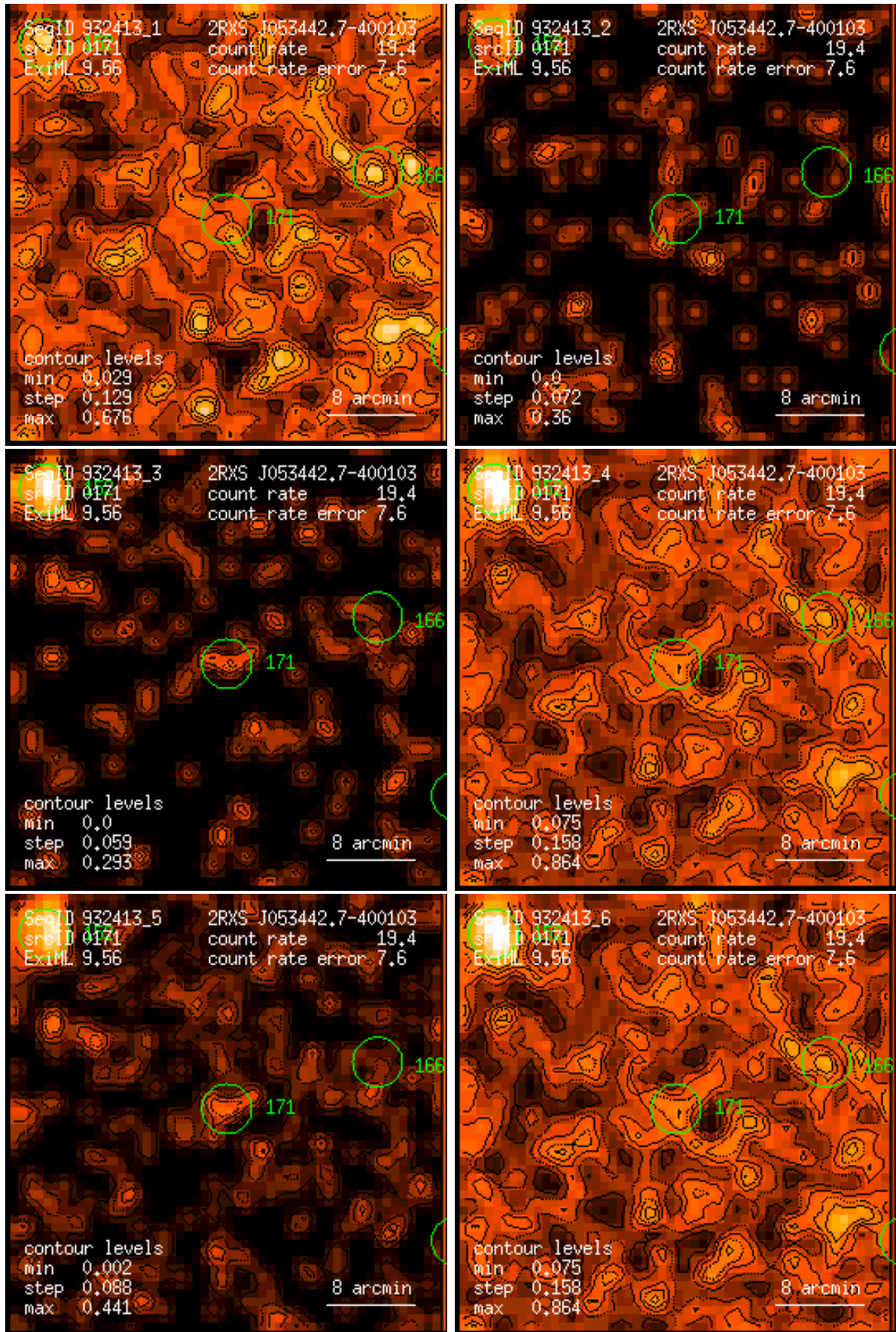
Figure 171: RASS 932413: detection 0171: band rate images, Gaussian filter: (1) PSPC channels 11 – 41, (2) 52 – 90, (3) 91 – 201, (4) 11 – 235, (5) 52 – 201, (6) 11 – 201. Broad band rates in counts/ks. Band rate contour levels in counts/ks/arcmin 2 .
