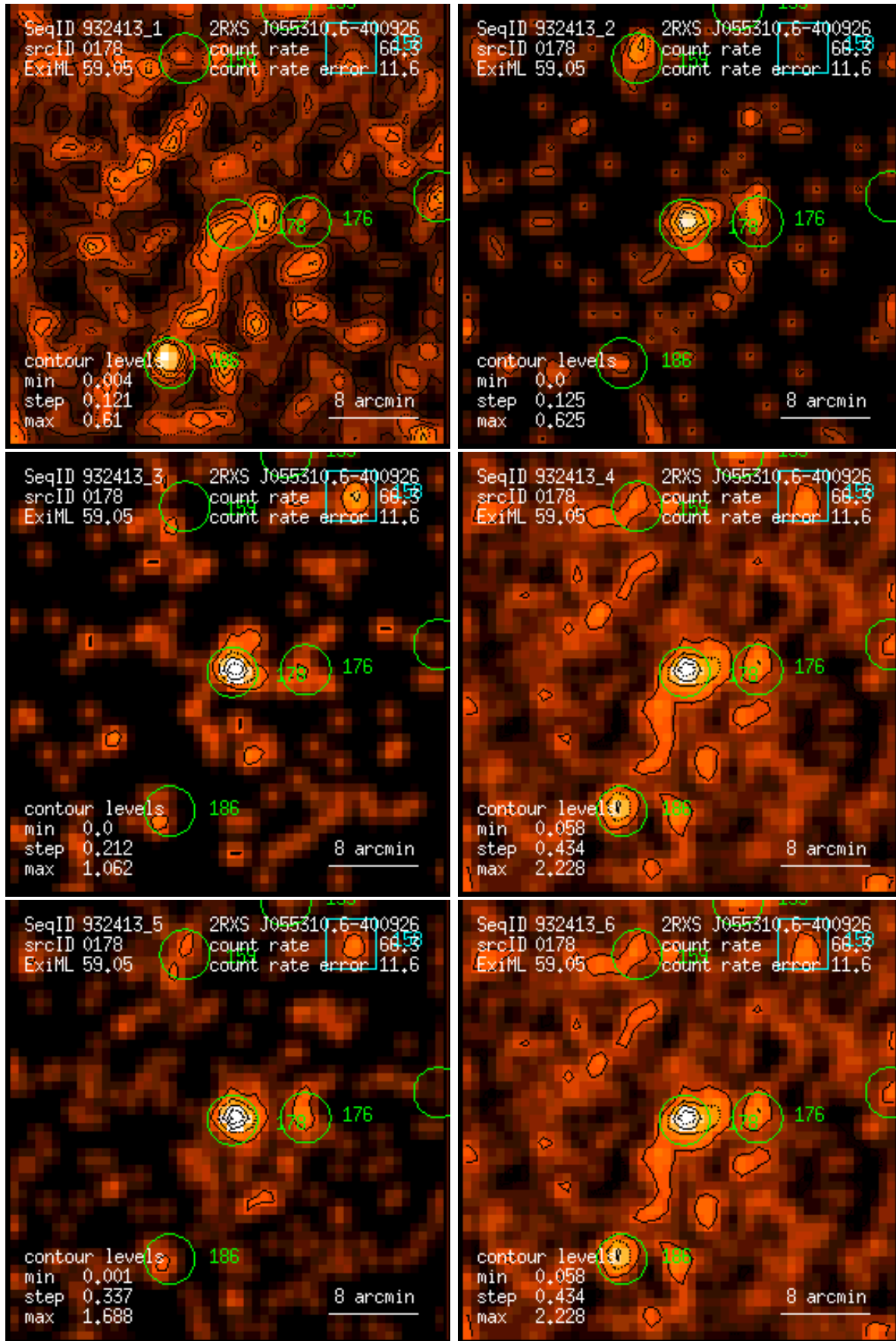
Figure 178: RASS 932413: detection 0178: band rate images, Gaussian filter: (1) PSPC channels 11 – 41, (2) 52 – 90, (3) 91 – 201, (4) 11 – 235, (5) 52 – 201, (6) 11 – 201. Broad band rates in counts/ks. Band rate contour levels in counts/ks/arcmin 2 .
