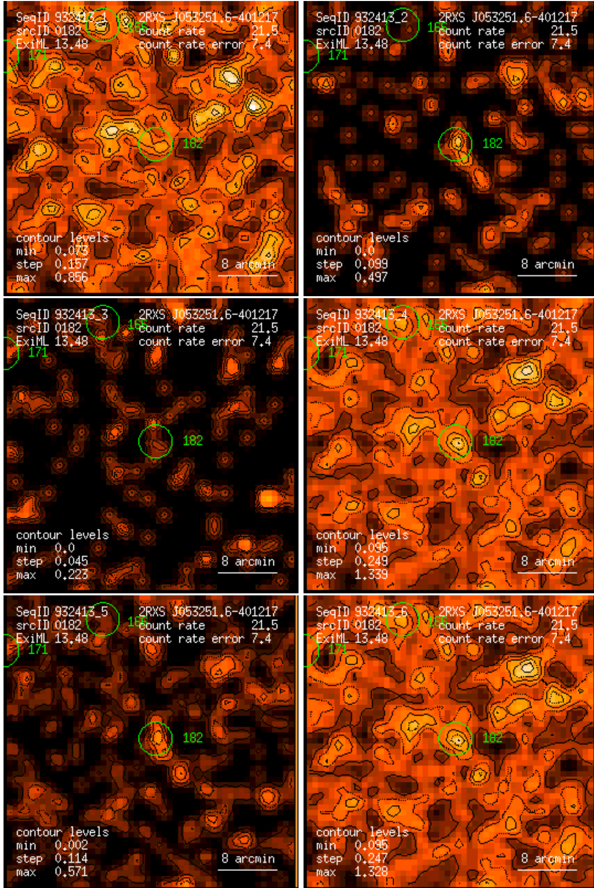
Figure 182: RASS 932413: detection 0182: band rate images, Gaussian filter: (1) PSPC channels 11 – 41, (2) 52 – 90, (3) 91 – 201, (4) 11 – 235, (5) 52 – 201, (6) 11 – 201. Broad band rates in counts/ks. Band rate contour levels in counts/ks/arcmin 2 .
