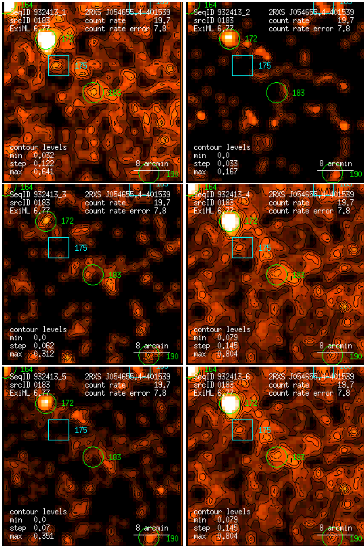
Figure 183: RASS 932413: detection 0183: band rate images, Gaussian filter: (1) PSPC channels 11 – 41, (2) 52 – 90, (3) 91 – 201, (4) 11 – 235, (5) 52 – 201, (6) 11 – 201. Broad band rates in counts/ks. Band rate contour levels in counts/ks/arcmin 2 .
