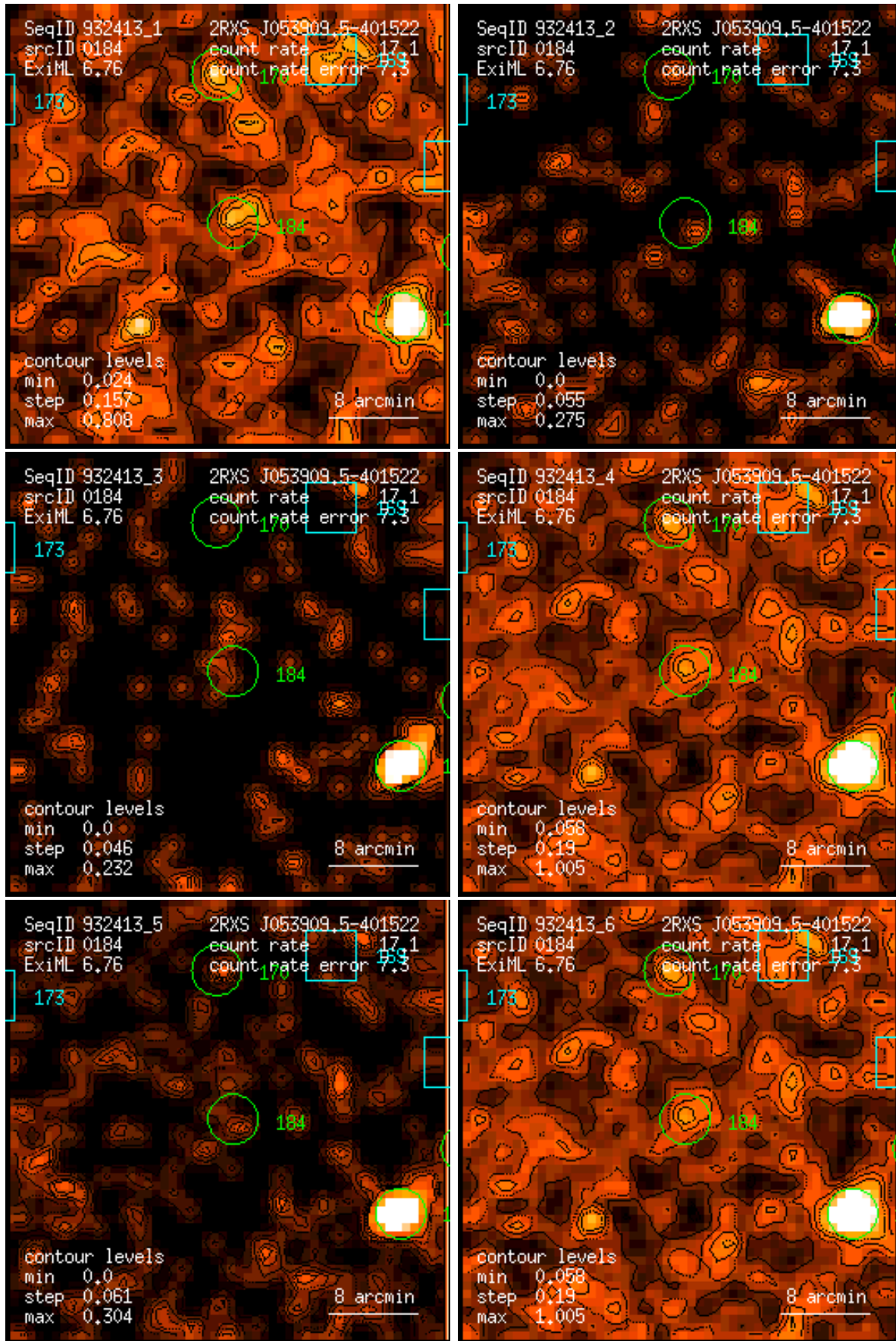
Figure 184: RASS 932413: detection 0184: band rate images, Gaussian filter: (1) PSPC channels 11 – 41, (2) 52 – 90, (3) 91 – 201, (4) 11 – 235, (5) 52 – 201, (6) 11 – 201. Broad band rates in counts/ks. Band rate contour levels in counts/ks/arcmin 2 .
