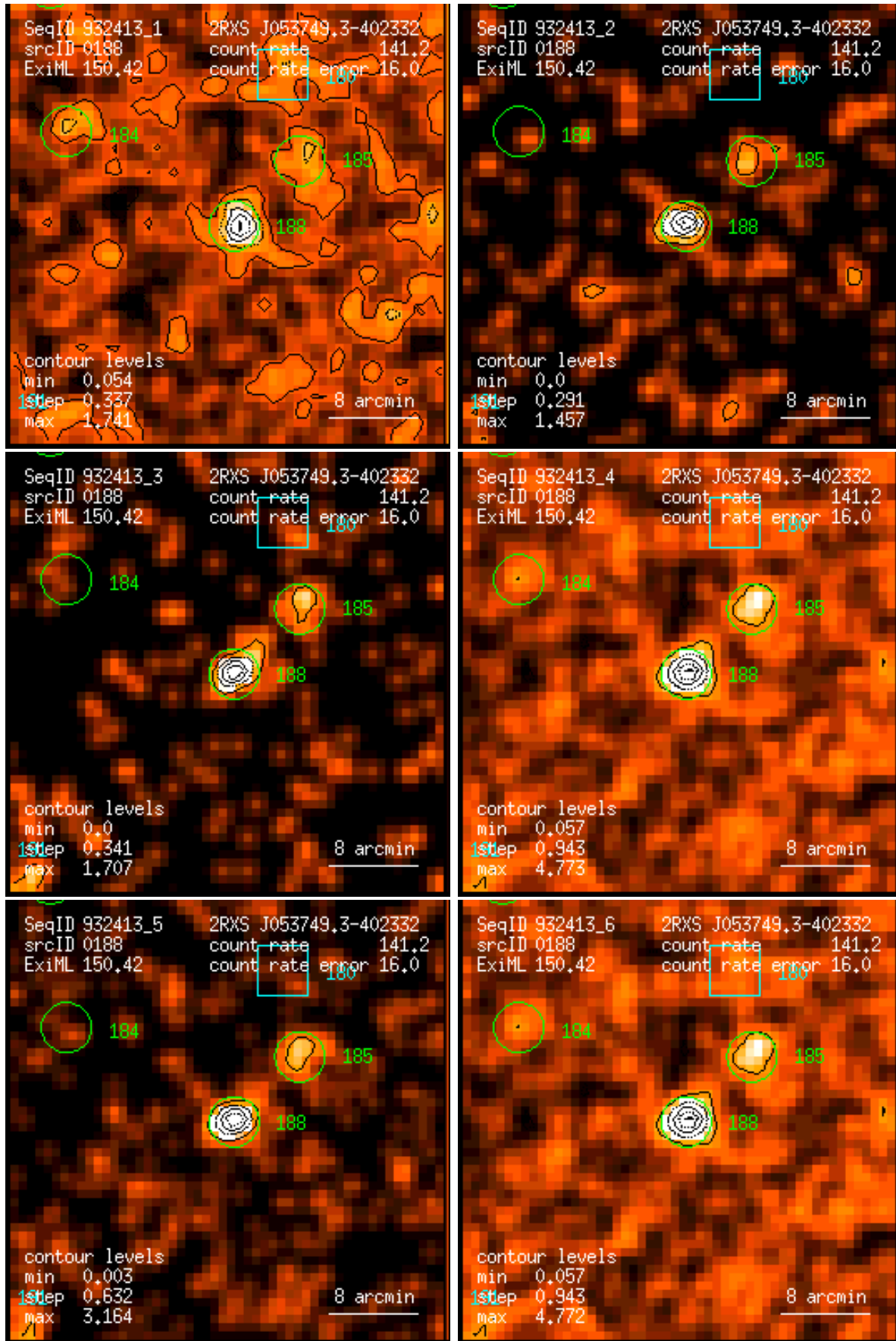
Figure 188: RASS 932413: detection 0188: band rate images, Gaussian filter: (1) PSPC channels 11 – 41, (2) 52 – 90, (3) 91 – 201, (4) 11 – 235, (5) 52 – 201, (6) 11 – 201. Broad band rates in counts/ks. Band rate contour levels in counts/ks/arcmin 2 .
