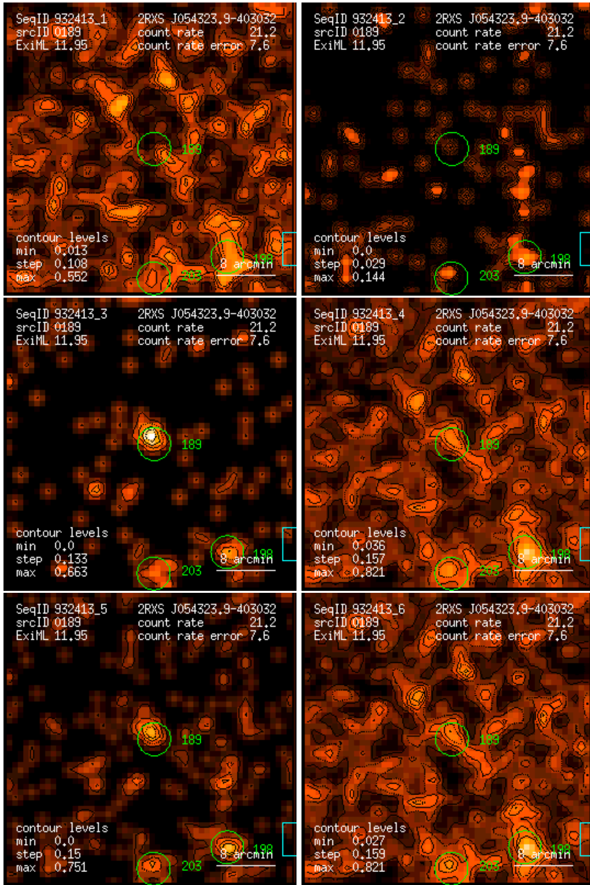
Figure 189: RASS 932413: detection 0189: band rate images, Gaussian filter: (1) PSPC channels 11 – 41, (2) 52 – 90, (3) 91 – 201, (4) 11 – 235, (5) 52 – 201, (6) 11 – 201. Broad band rates in counts/ks. Band rate contour levels in counts/ks/arcmin 2 .
