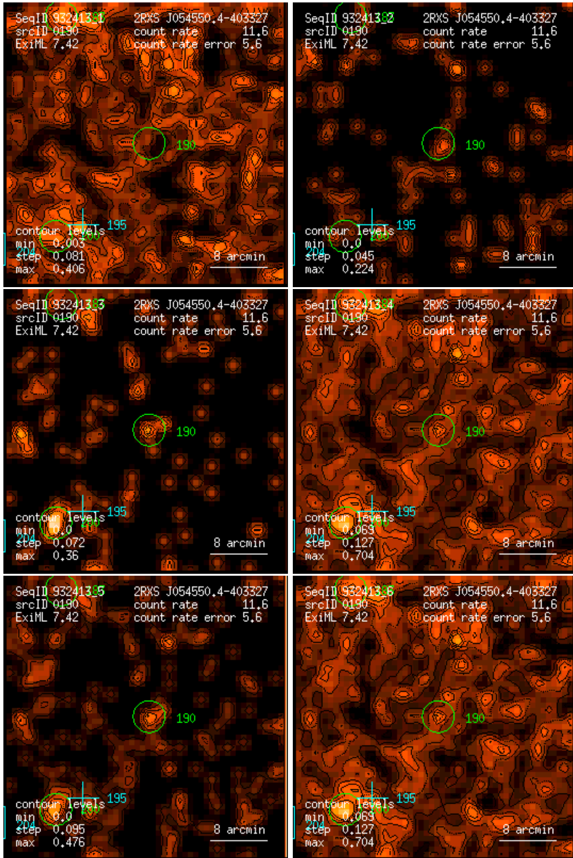
Figure 190: RASS 932413: detection 0190: band rate images, Gaussian filter: (1) PSPC channels 11 – 41, (2) 52 – 90, (3) 91 – 201, (4) 11 – 235, (5) 52 – 201, (6) 11 – 201. Broad band rates in counts/ks. Band rate contour levels in counts/ks/arcmin 2 .
