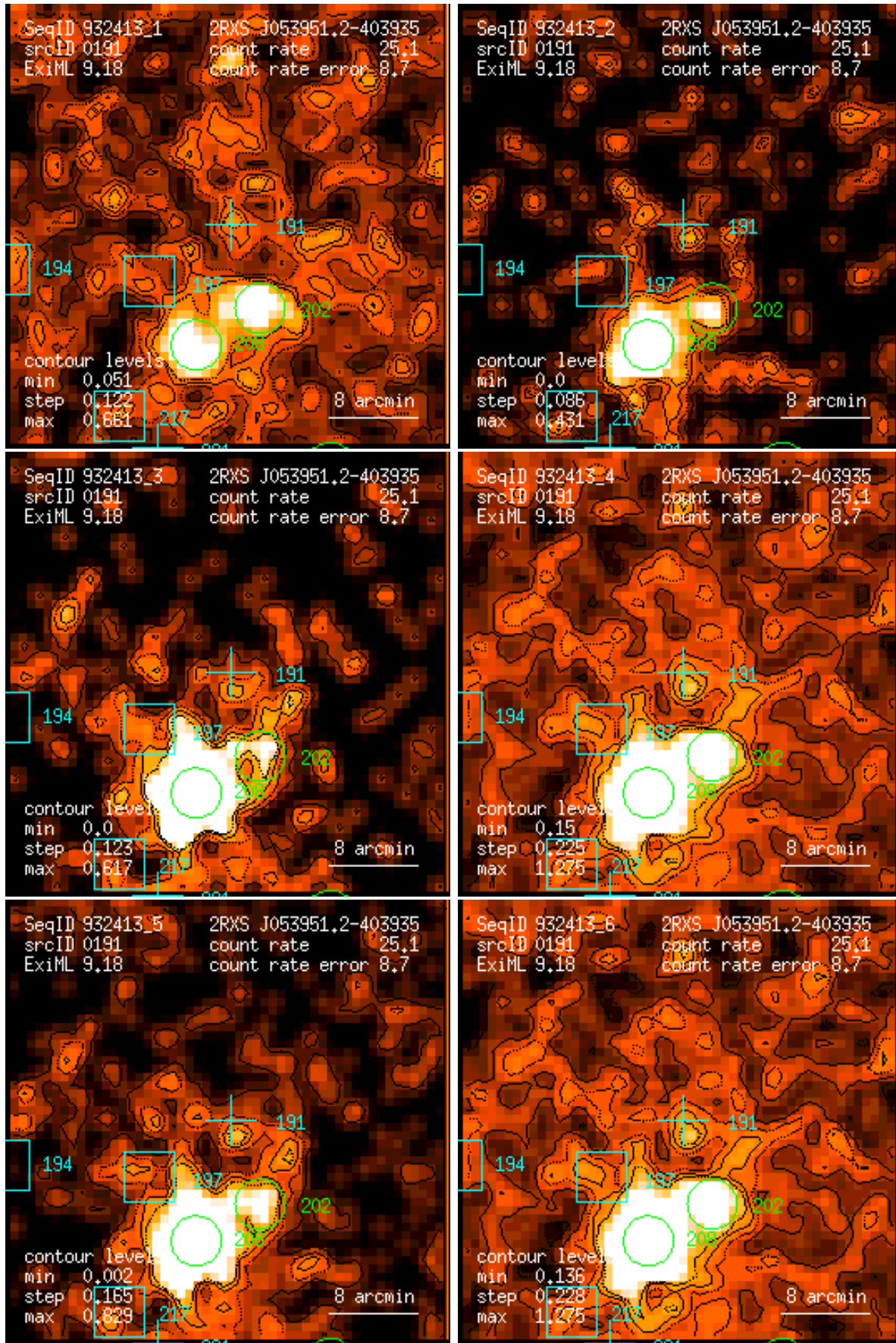
Figure 191: RASS 932413: detection 0191: band rate images, Gaussian filter: (1) PSPC channels 11 – 41, (2) 52 – 90, (3) 91 – 201, (4) 11 – 235, (5) 52 – 201, (6) 11 – 201. Broad band rates in counts/ks. Band rate contour levels in counts/ks/arcmin 2 .
