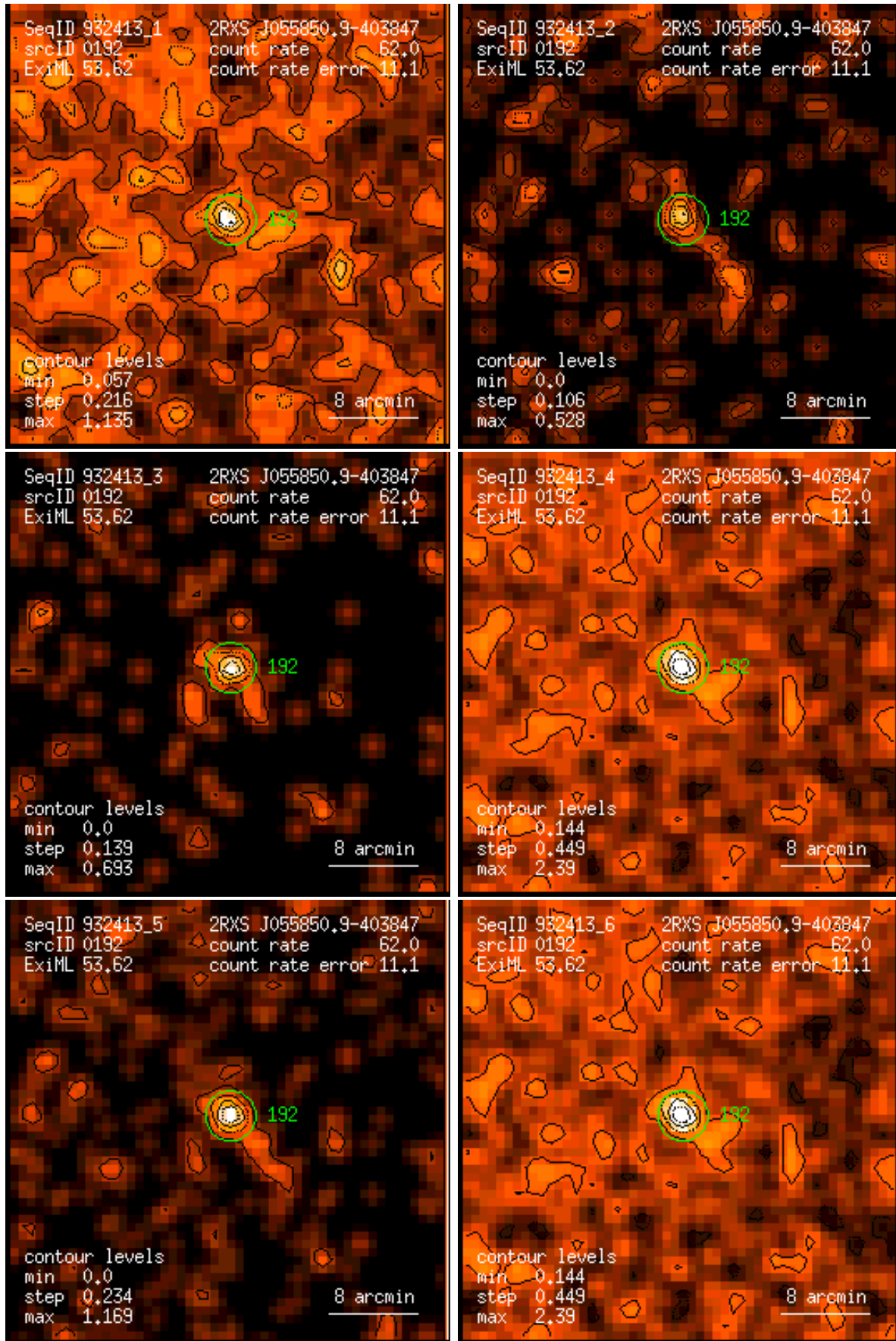
Figure 192: RASS 932413: detection 0192: band rate images, Gaussian filter: (1) PSPC channels 11 – 41, (2) 52 – 90, (3) 91 – 201, (4) 11 – 235, (5) 52 – 201, (6) 11 – 201. Broad band rates in counts/ks. Band rate contour levels in counts/ks/arcmin 2 .
