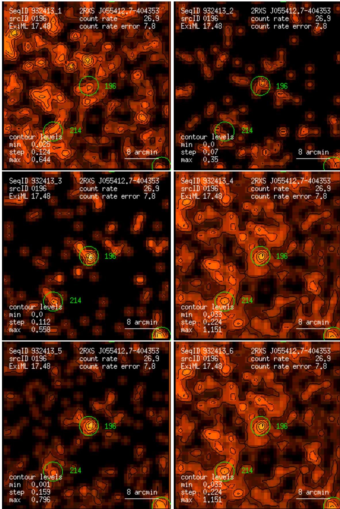
Figure 196: RASS 932413: detection 0196: band rate images, Gaussian filter: (1) PSPC channels 11 – 41, (2) 52 – 90, (3) 91 – 201, (4) 11 – 235, (5) 52 – 201, (6) 11 – 201. Broad band rates in counts/ks. Band rate contour levels in counts/ks/arcmin 2 .
