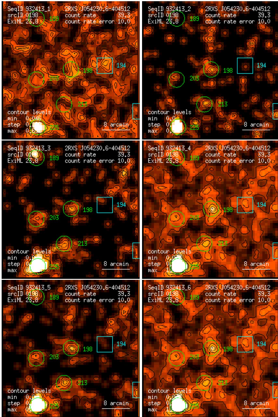
Figure 198: RASS 932413: detection 0198: band rate images, Gaussian filter: (1) PSPC channels 11 – 41, (2) 52 – 90, (3) 91 – 201, (4) 11 – 235, (5) 52 – 201, (6) 11 – 201. Broad band rates in counts/ks. Band rate contour levels in counts/ks/arcmin 2 .
