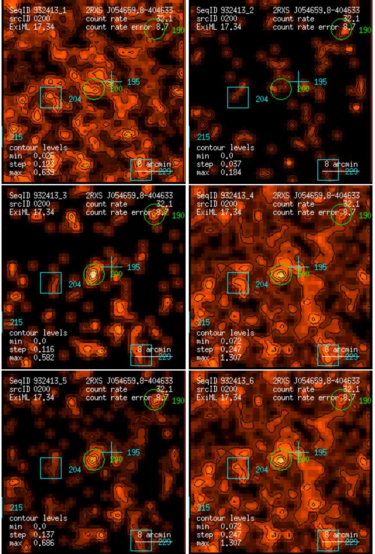
Figure 200: RASS 932413: detection 0200: band rate images, Gaussian filter: (1) PSPC channels 11 – 41, (2) 52 – 90, (3) 91 – 201, (4) 11 – 235, (5) 52 – 201, (6) 11 – 201. Broad band rates in counts/ks. Band rate contour levels in counts/ks/arcmin 2 .
