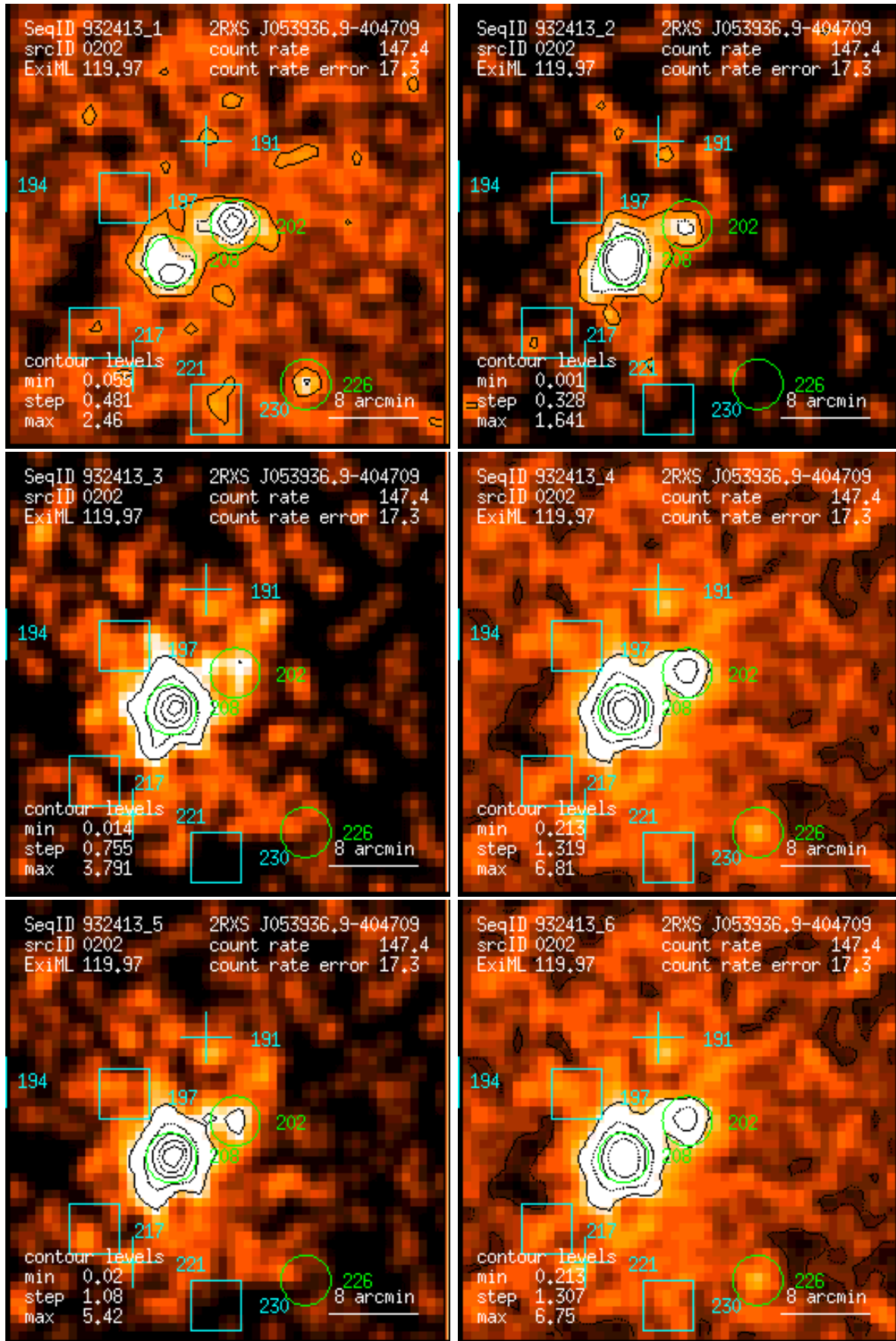
Figure 202: RASS 932413: detection 0202: band rate images, Gaussian filter: (1) PSPC channels 11 – 41, (2) 52 – 90, (3) 91 – 201, (4) 11 – 235, (5) 52 – 201, (6) 11 – 201. Broad band rates in counts/ks. Band rate contour levels in counts/ks/arcmin 2 .
