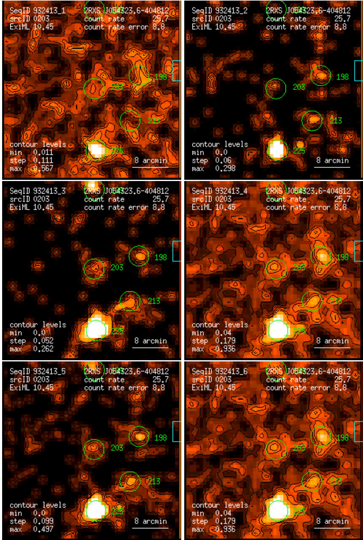
Figure 203: RASS 932413: detection 0203: band rate images, Gaussian filter: (1) PSPC channels 11 – 41, (2) 52 – 90, (3) 91 – 201, (4) 11 – 235, (5) 52 – 201, (6) 11 – 201. Broad band rates in counts/ks. Band rate contour levels in counts/ks/arcmin 2 .
