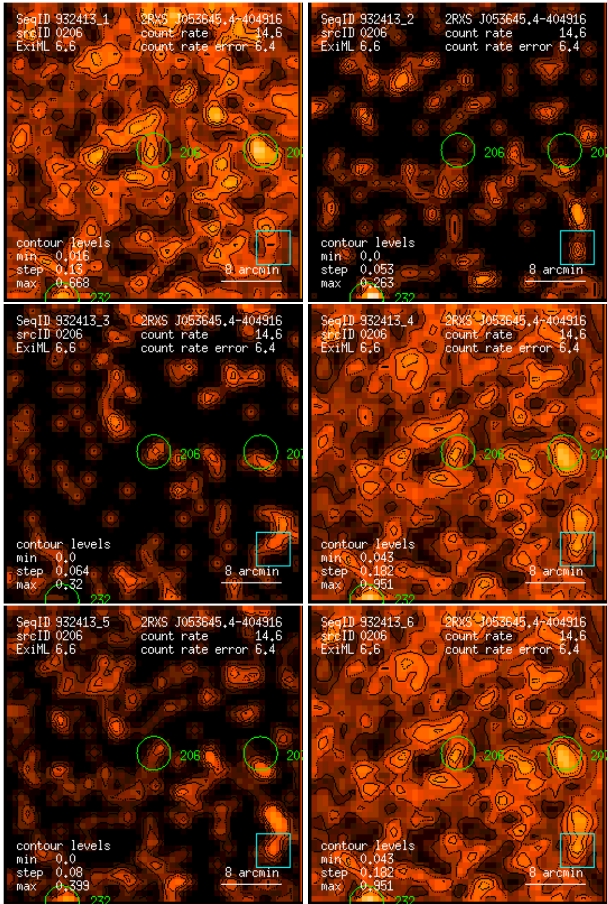
Figure 206: RASS 932413: detection 0206: band rate images, Gaussian filter: (1) PSPC channels 11 – 41, (2) 52 – 90, (3) 91 – 201, (4) 11 – 235, (5) 52 – 201, (6) 11 – 201. Broad band rates in counts/ks. Band rate contour levels in counts/ks/arcmin 2 .
