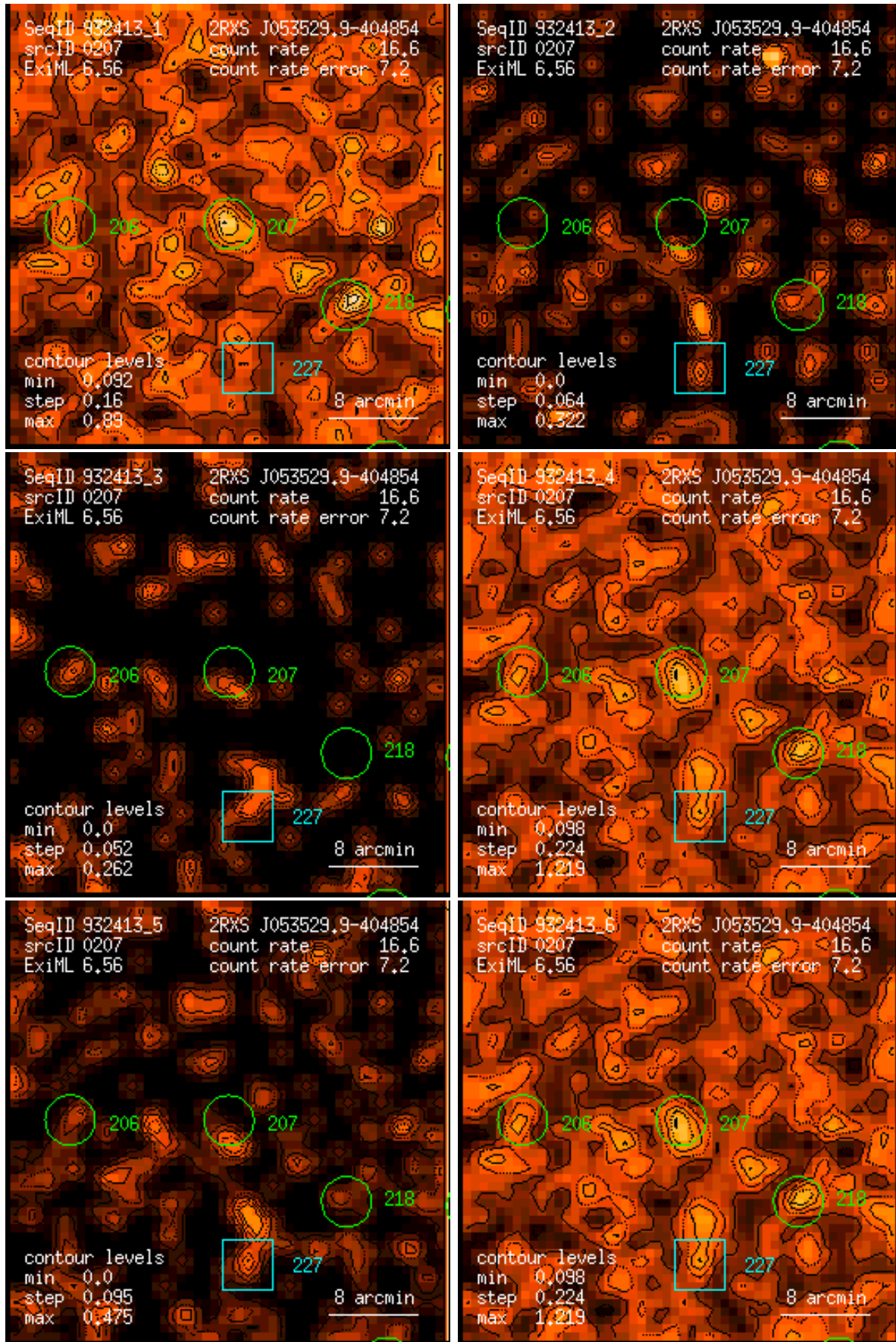
Figure 207: RASS 932413: detection 0207: band rate images, Gaussian filter: (1) PSPC channels 11 – 41, (2) 52 – 90, (3) 91 – 201, (4) 11 – 235, (5) 52 – 201, (6) 11 – 201. Broad band rates in counts/ks. Band rate contour levels in counts/ks/arcmin 2 .
