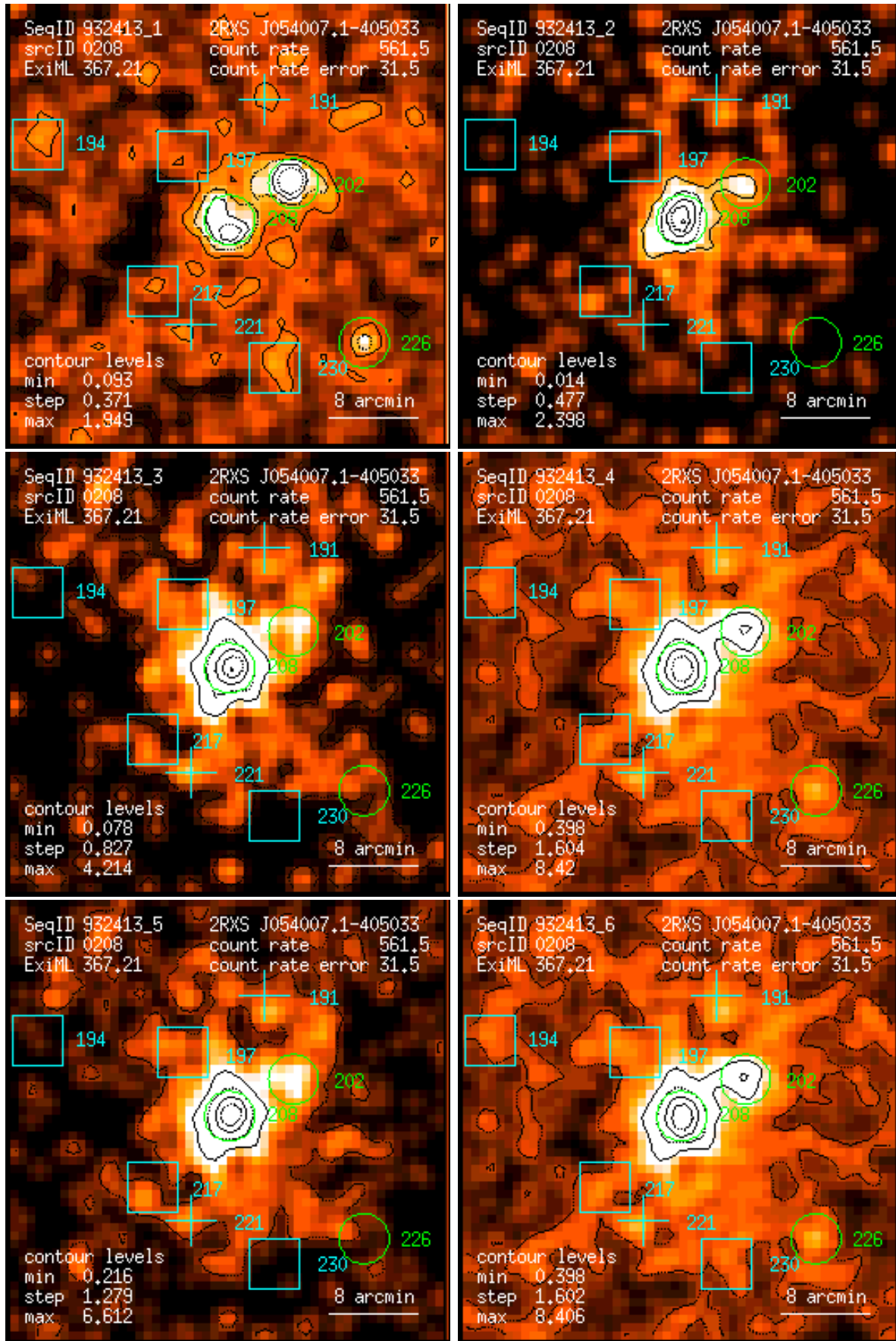
Figure 208: RASS 932413: detection 0208: band rate images, Gaussian filter: (1) PSPC channels 11 – 41, (2) 52 – 90, (3) 91 – 201, (4) 11 – 235, (5) 52 – 201, (6) 11 – 201. Broad band rates in counts/ks. Band rate contour levels in counts/ks/arcmin 2 .
