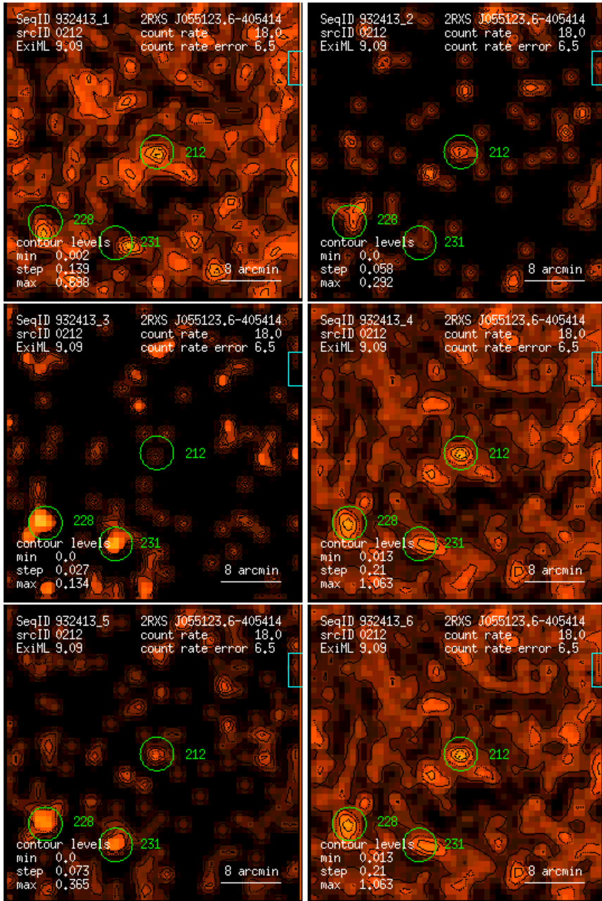
Figure 212: RASS 932413: detection 0212: band rate images, Gaussian filter: (1) PSPC channels 11 – 41, (2) 52 – 90, (3) 91 – 201, (4) 11 – 235, (5) 52 – 201, (6) 11 – 201. Broad band rates in counts/ks. Band rate contour levels in counts/ks/arcmin 2 .
