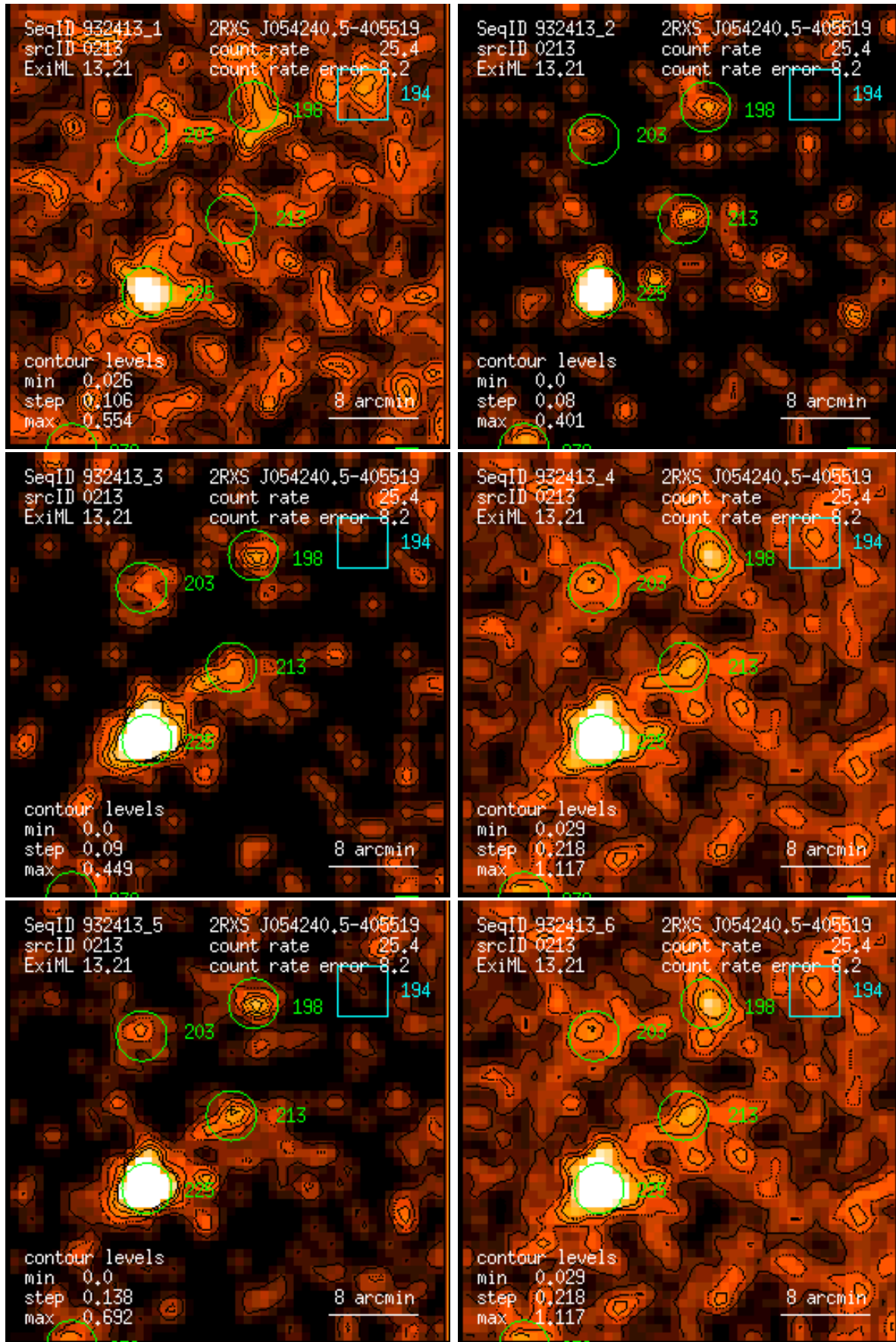
Figure 213: RASS 932413: detection 0213: band rate images, Gaussian filter: (1) PSPC channels 11 – 41, (2) 52 – 90, (3) 91 – 201, (4) 11 – 235, (5) 52 – 201, (6) 11 – 201. Broad band rates in counts/ks. Band rate contour levels in counts/ks/arcmin 2 .
