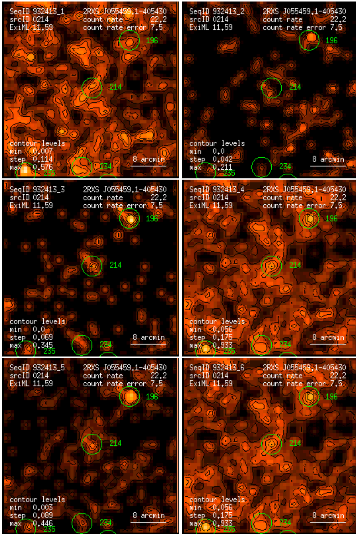
Figure 214: RASS 932413: detection 0214: band rate images, Gaussian filter: (1) PSPC channels 11 – 41, (2) 52 – 90, (3) 91 – 201, (4) 11 – 235, (5) 52 – 201, (6) 11 – 201. Broad band rates in counts/ks. Band rate contour levels in counts/ks/arcmin 2 .
