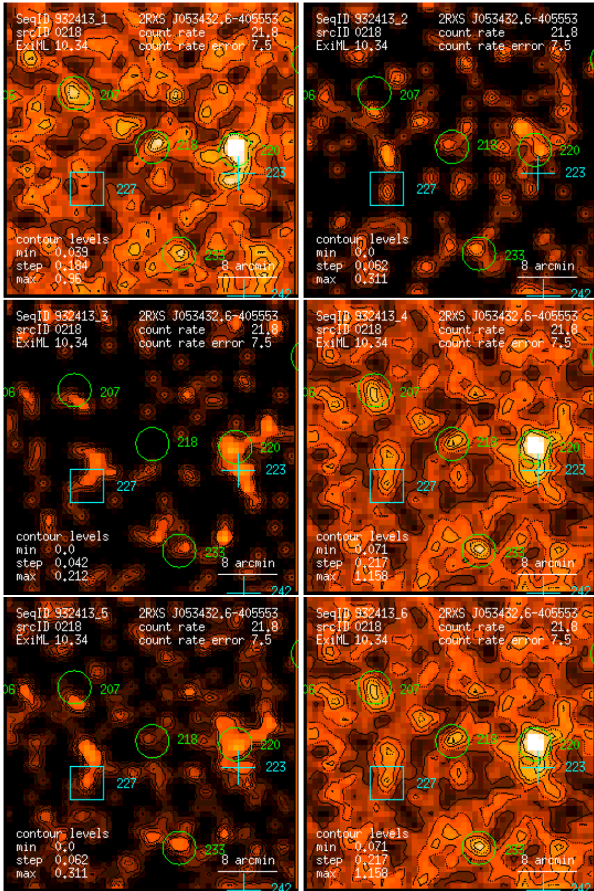
Figure 218: RASS 932413: detection 0218: band rate images, Gaussian filter: (1) PSPC channels 11 – 41, (2) 52 – 90, (3) 91 – 201, (4) 11 – 235, (5) 52 – 201, (6) 11 – 201. Broad band rates in counts/ks. Band rate contour levels in counts/ks/arcmin 2 .
