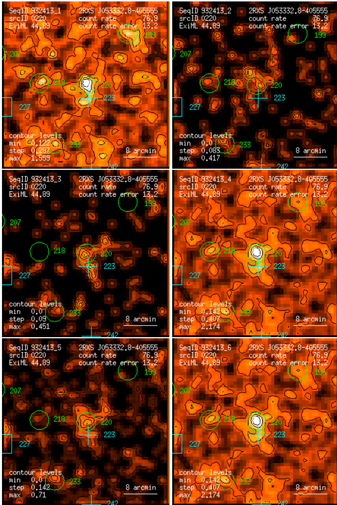
Figure 220: RASS 932413: detection 0220: band rate images, Gaussian filter: (1) PSPC channels 11 – 41, (2) 52 – 90, (3) 91 – 201, (4) 11 – 235, (5) 52 – 201, (6) 11 – 201. Broad band rates in counts/ks. Band rate contour levels in counts/ks/arcmin 2 .
