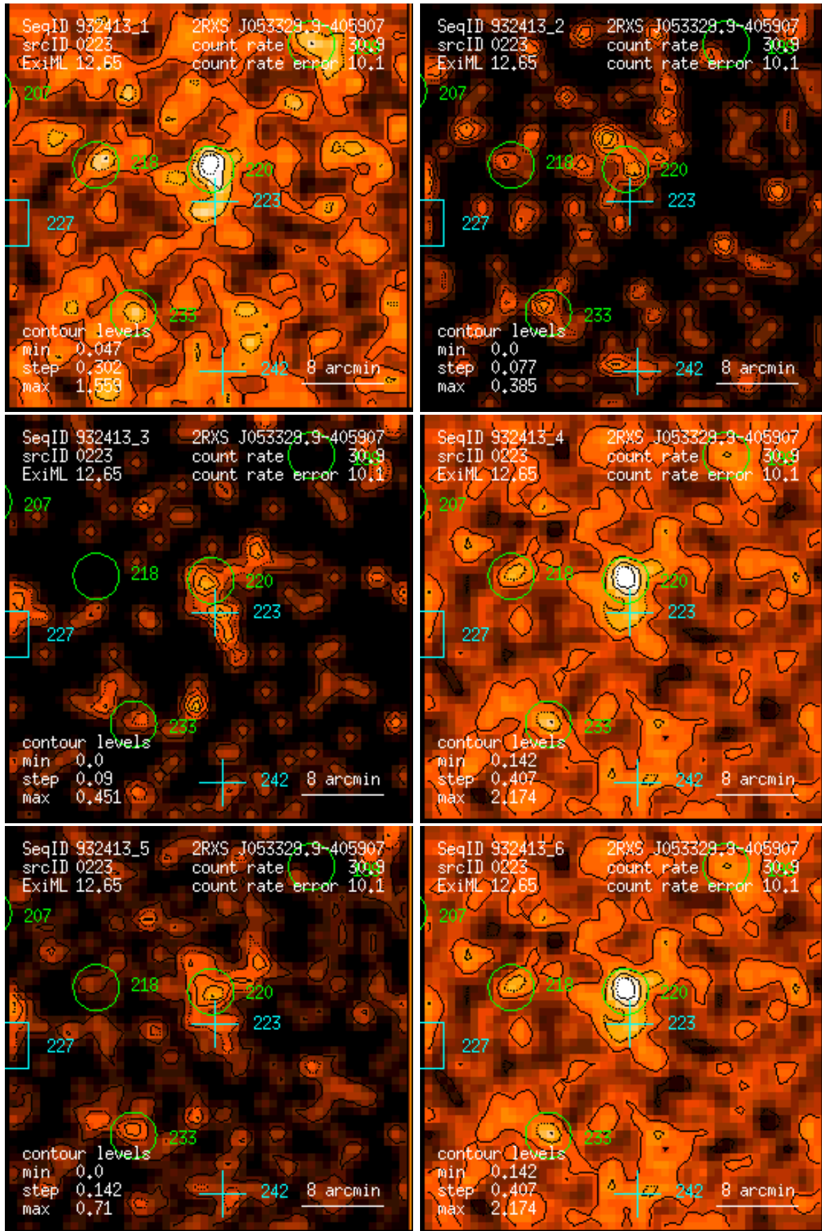
Figure 223: RASS 932413: detection 0223: band rate images, Gaussian filter: (1) PSPC channels 11 – 41, (2) 52 – 90, (3) 91 – 201, (4) 11 – 235, (5) 52 – 201, (6) 11 – 201. Broad band rates in counts/ks. Band rate contour levels in counts/ks/arcmin 2 .
