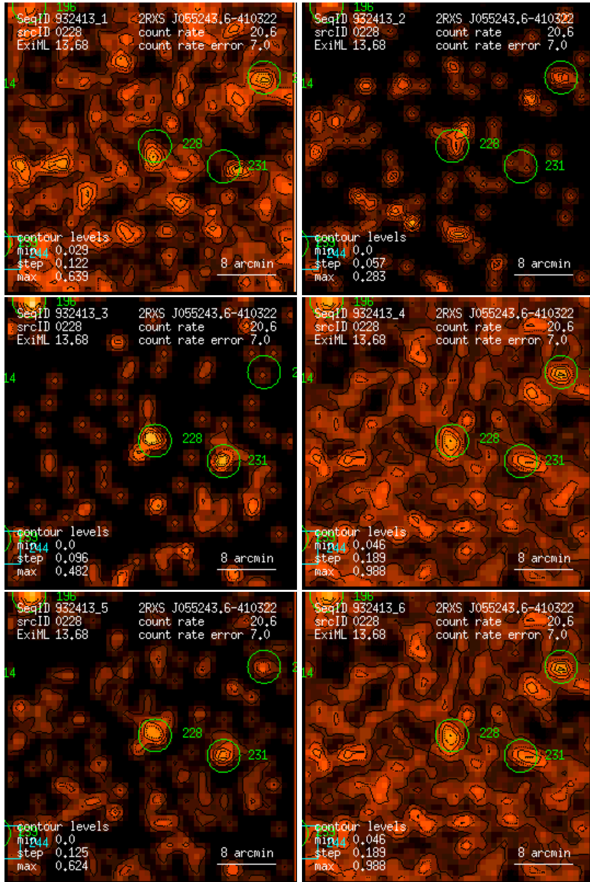
Figure 228: RASS 932413: detection 0228: band rate images, Gaussian filter: (1) PSPC channels 11 – 41, (2) 52 – 90, (3) 91 – 201, (4) 11 – 235, (5) 52 – 201, (6) 11 – 201. Broad band rates in counts/ks. Band rate contour levels in counts/ks/arcmin 2 .
