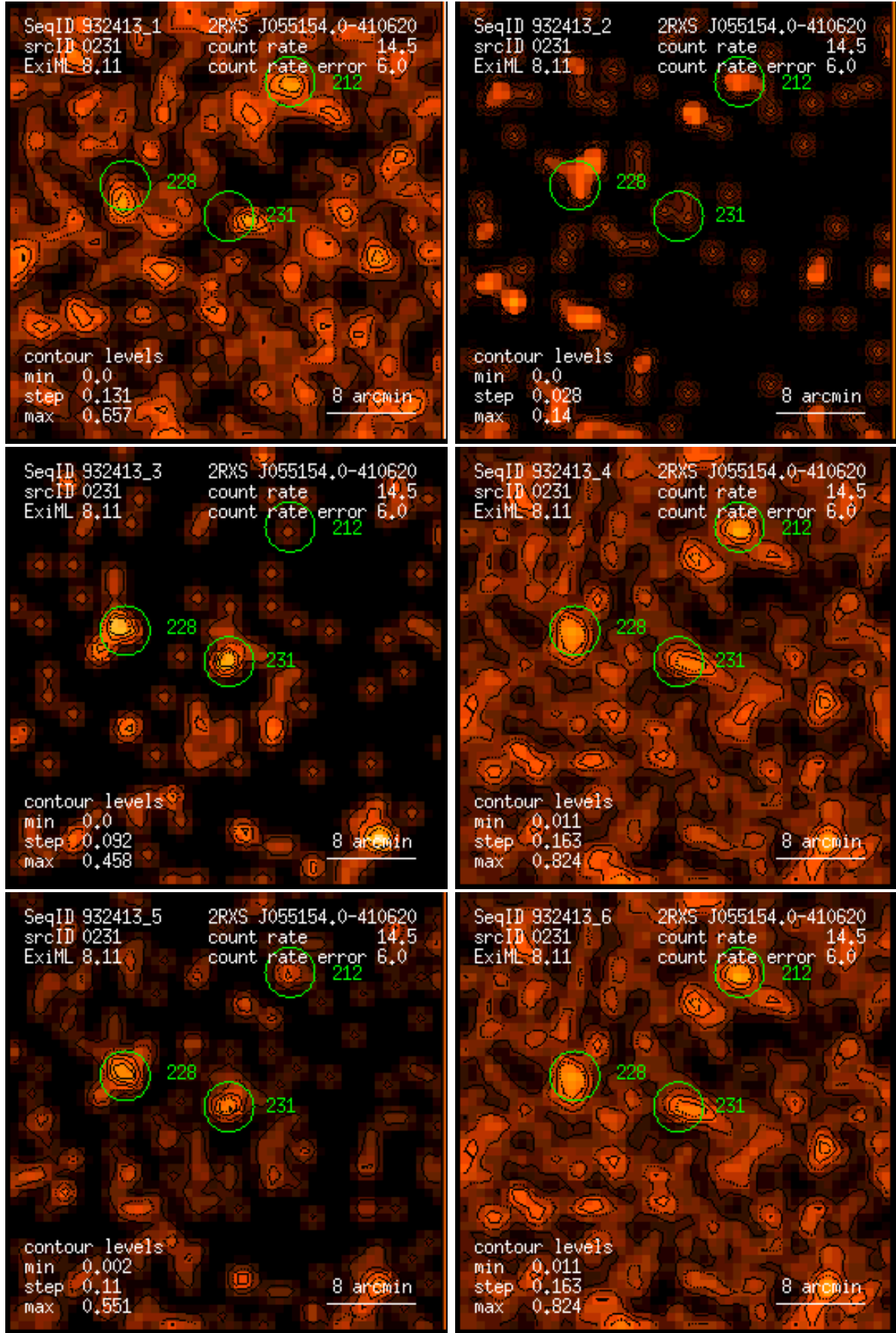
Figure 231: RASS 932413: detection 0231: band rate images, Gaussian filter: (1) PSPC channels 11 – 41, (2) 52 – 90, (3) 91 – 201, (4) 11 – 235, (5) 52 – 201, (6) 11 – 201. Broad band rates in counts/ks. Band rate contour levels in counts/ks/arcmin 2 .
