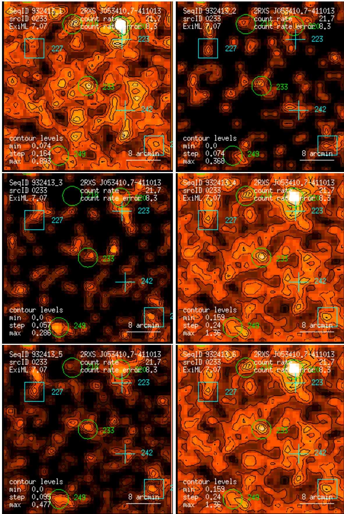
Figure 233: RASS 932413: detection 0233: band rate images, Gaussian filter: (1) PSPC channels 11 – 41, (2) 52 – 90, (3) 91 – 201, (4) 11 – 235, (5) 52 – 201, (6) 11 – 201. Broad band rates in counts/ks. Band rate contour levels in counts/ks/arcmin 2 .
