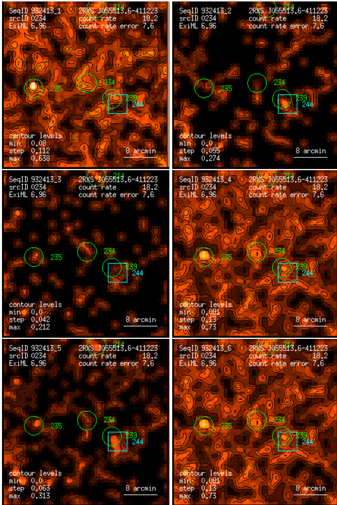
Figure 234: RASS 932413: detection 0234: band rate images, Gaussian filter: (1) PSPC channels 11 – 41, (2) 52 – 90, (3) 91 – 201, (4) 11 – 235, (5) 52 – 201, (6) 11 – 201. Broad band rates in counts/ks. Band rate contour levels in counts/ks/arcmin 2 .
