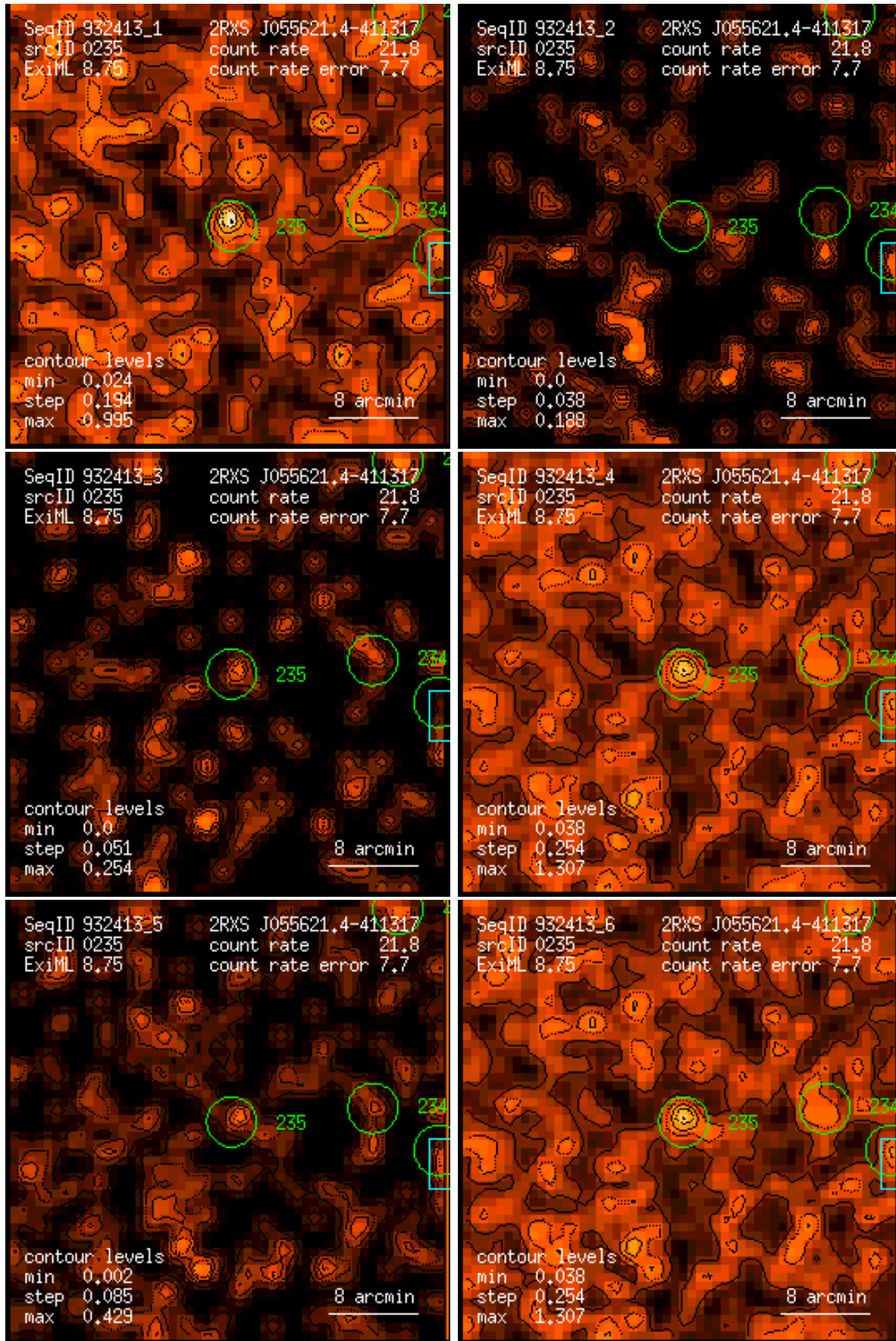
Figure 235: RASS 932413: detection 0235: band rate images, Gaussian filter: (1) PSPC channels 11 – 41, (2) 52 – 90, (3) 91 – 201, (4) 11 – 235, (5) 52 – 201, (6) 11 – 201. Broad band rates in counts/ks. Band rate contour levels in counts/ks/arcmin 2 .
