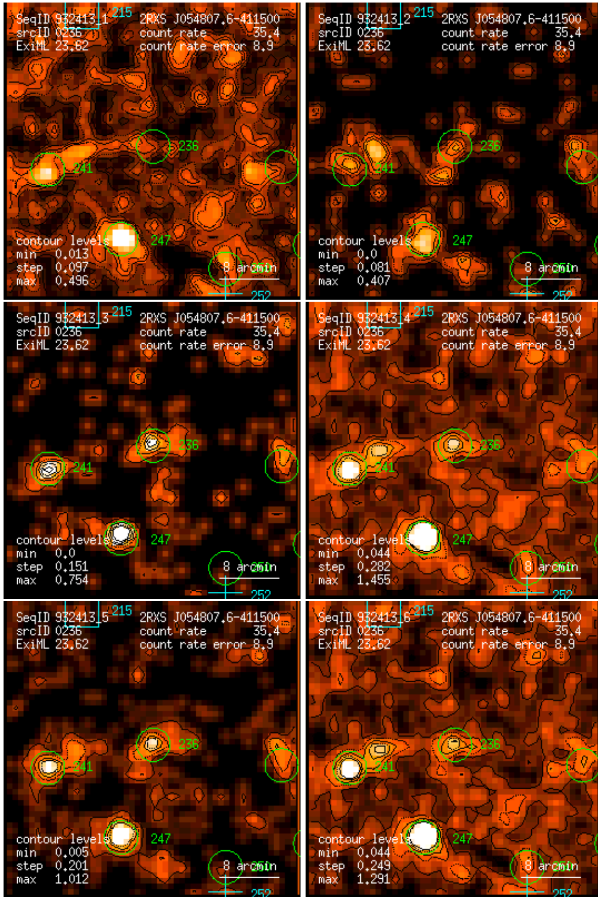
Figure 236: RASS 932413: detection 0236: band rate images, Gaussian filter: (1) PSPC channels 11 – 41, (2) 52 – 90, (3) 91 – 201, (4) 11 – 235, (5) 52 – 201, (6) 11 – 201. Broad band rates in counts/ks. Band rate contour levels in counts/ks/arcmin 2 .
