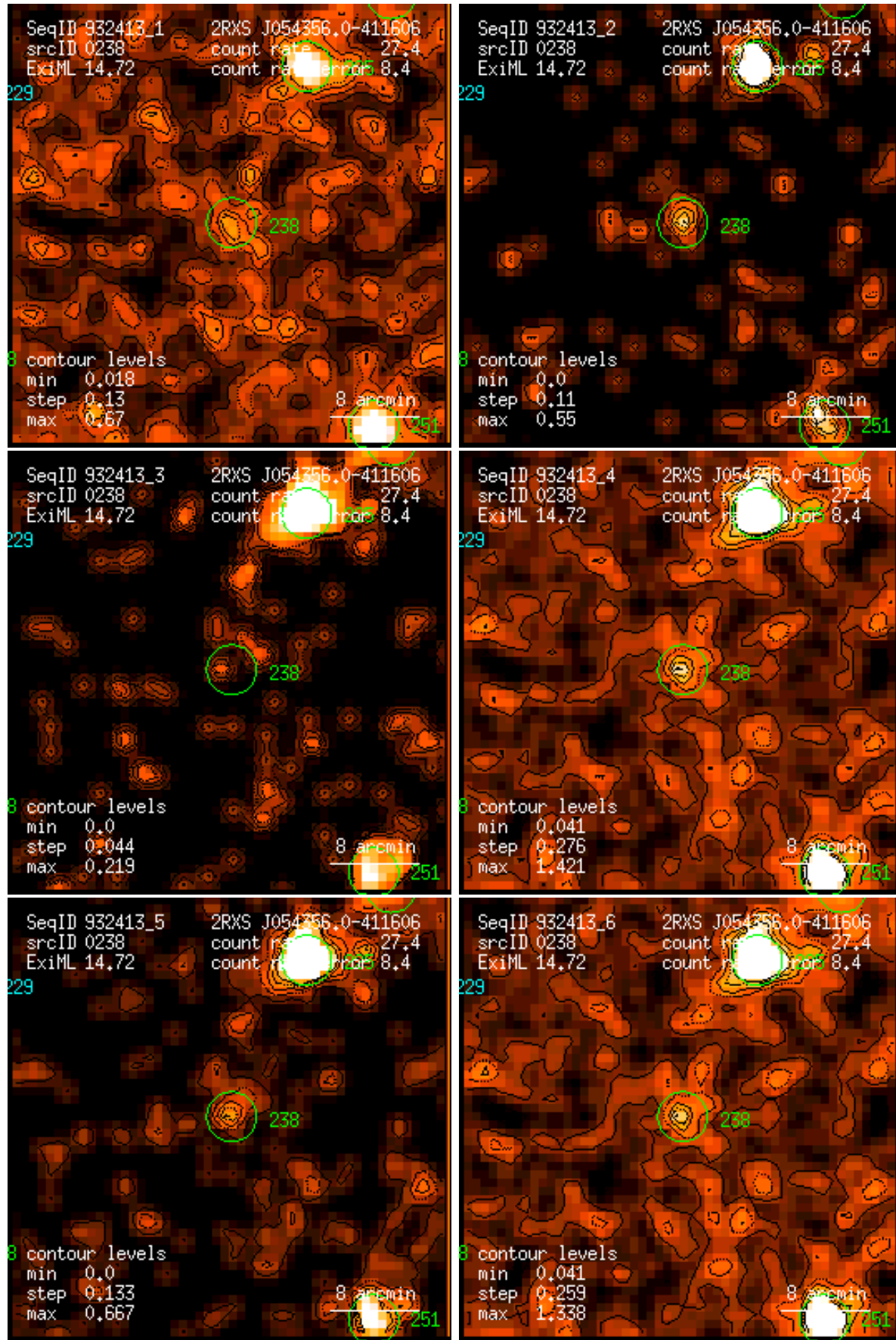
Figure 238: RASS 932413: detection 0238: band rate images, Gaussian filter: (1) PSPC channels 11 – 41, (2) 52 – 90, (3) 91 – 201, (4) 11 – 235, (5) 52 – 201, (6) 11 – 201. Broad band rates in counts/ks. Band rate contour levels in counts/ks/arcmin 2 .
