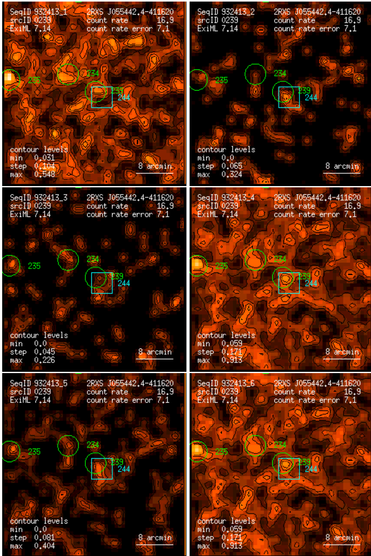
Figure 239: RASS 932413: detection 0239: band rate images, Gaussian filter: (1) PSPC channels 11 – 41, (2) 52 – 90, (3) 91 – 201, (4) 11 – 235, (5) 52 – 201, (6) 11 – 201. Broad band rates in counts/ks. Band rate contour levels in counts/ks/arcmin 2 .
