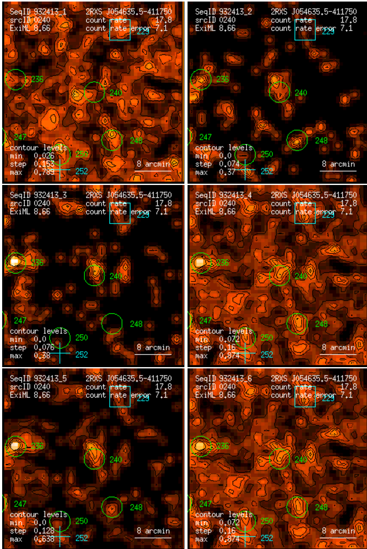
Figure 240: RASS 932413: detection 0240: band rate images, Gaussian filter: (1) PSPC channels 11 – 41, (2) 52 – 90, (3) 91 – 201, (4) 11 – 235, (5) 52 – 201, (6) 11 – 201. Broad band rates in counts/ks. Band rate contour levels in counts/ks/arcmin 2 .
