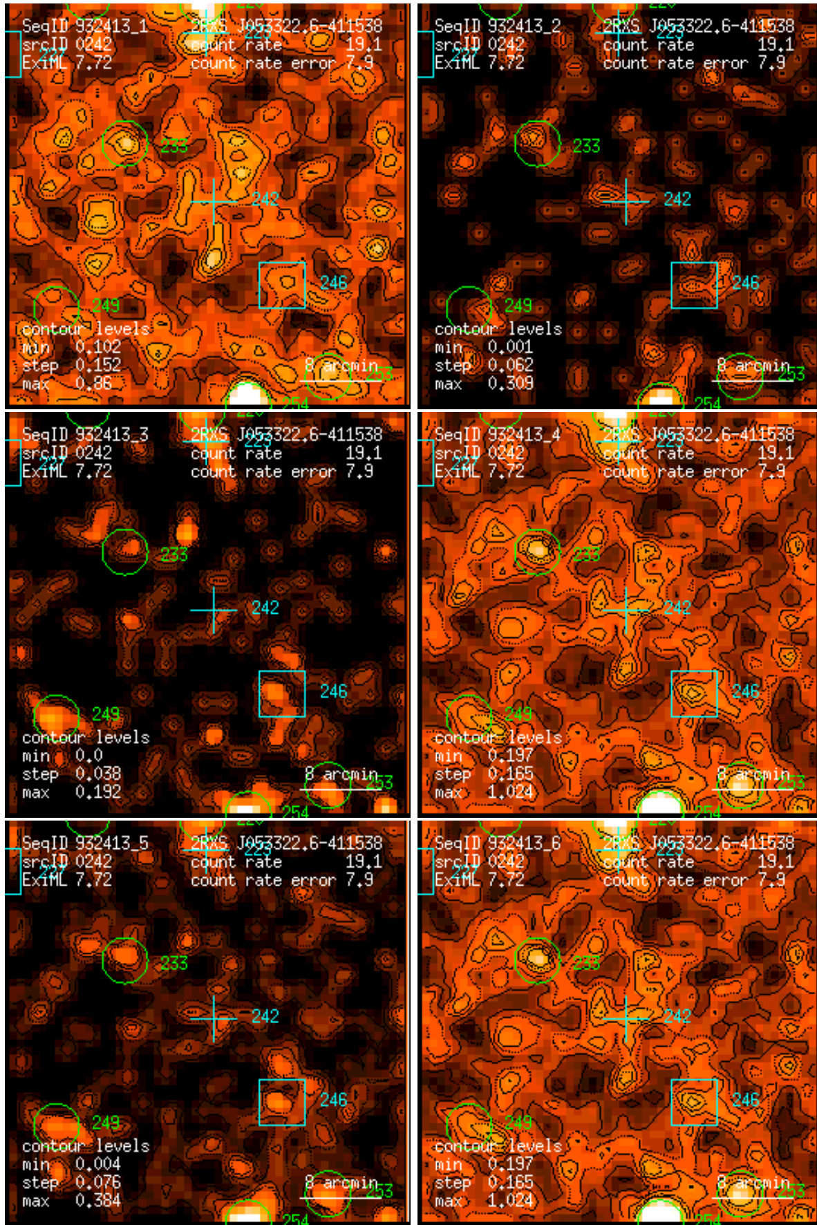
Figure 242: RASS 932413: detection 0242: band rate images, Gaussian filter: (1) PSPC channels 11 – 41, (2) 52 – 90, (3) 91 – 201, (4) 11 – 235, (5) 52 – 201, (6) 11 – 201. Broad band rates in counts/ks. Band rate contour levels in counts/ks/arcmin 2 .
