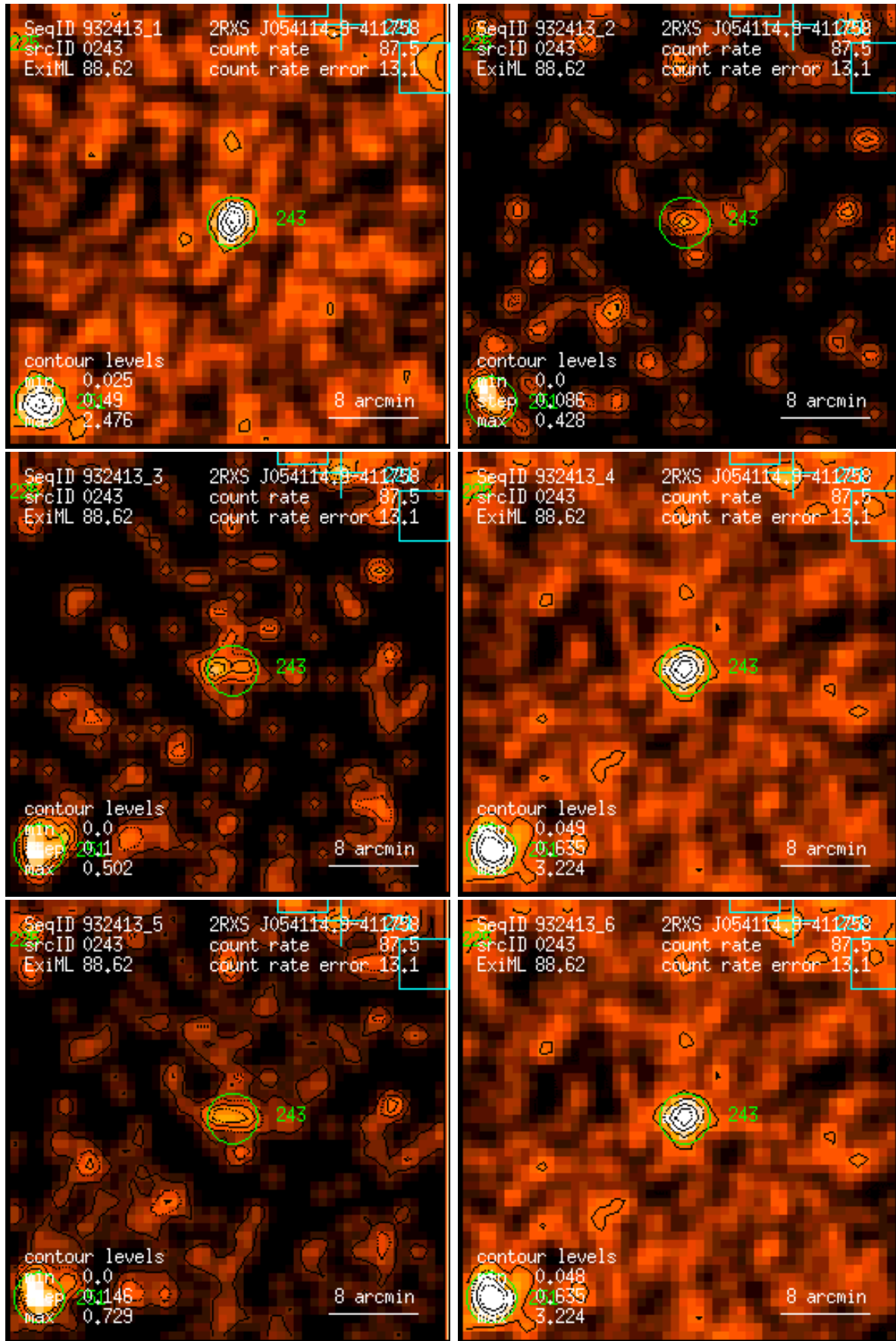
Figure 243: RASS 932413: detection 0243: band rate images, Gaussian filter: (1) PSPC channels 11 – 41, (2) 52 – 90, (3) 91 – 201, (4) 11 – 235, (5) 52 – 201, (6) 11 – 201. Broad band rates in counts/ks. Band rate contour levels in counts/ks/arcmin 2 .
