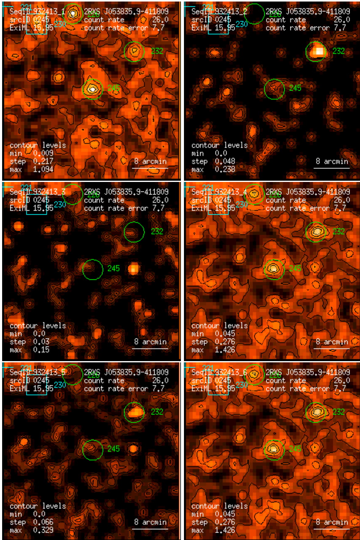
Figure 245: RASS 932413: detection 0245: band rate images, Gaussian filter: (1) PSPC channels 11 – 41, (2) 52 – 90, (3) 91 – 201, (4) 11 – 235, (5) 52 – 201, (6) 11 – 201. Broad band rates in counts/ks. Band rate contour levels in counts/ks/arcmin 2 .
