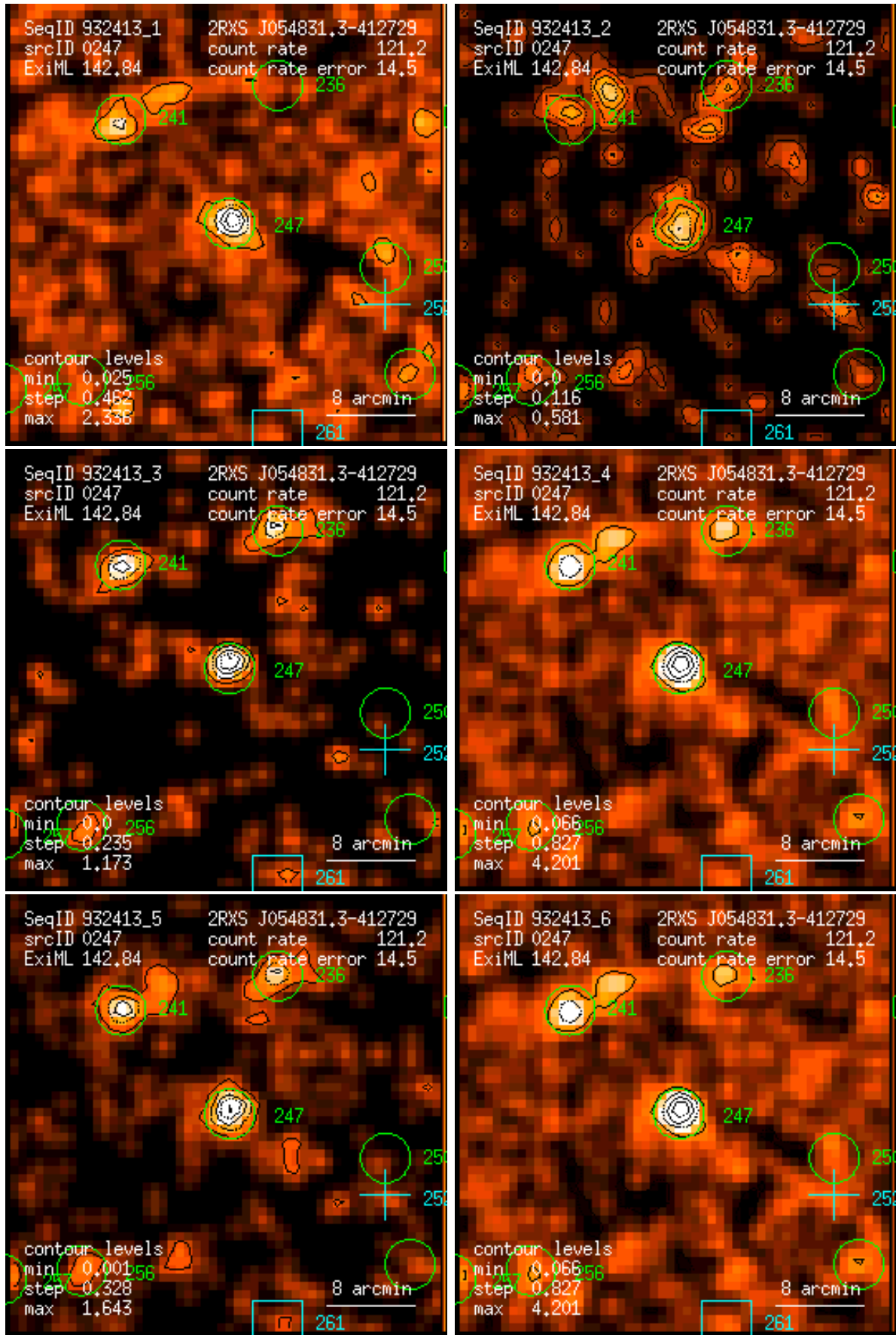
Figure 247: RASS 932413: detection 0247: band rate images, Gaussian filter: (1) PSPC channels 11 – 41, (2) 52 – 90, (3) 91 – 201, (4) 11 – 235, (5) 52 – 201, (6) 11 – 201. Broad band rates in counts/ks. Band rate contour levels in counts/ks/arcmin 2 .
