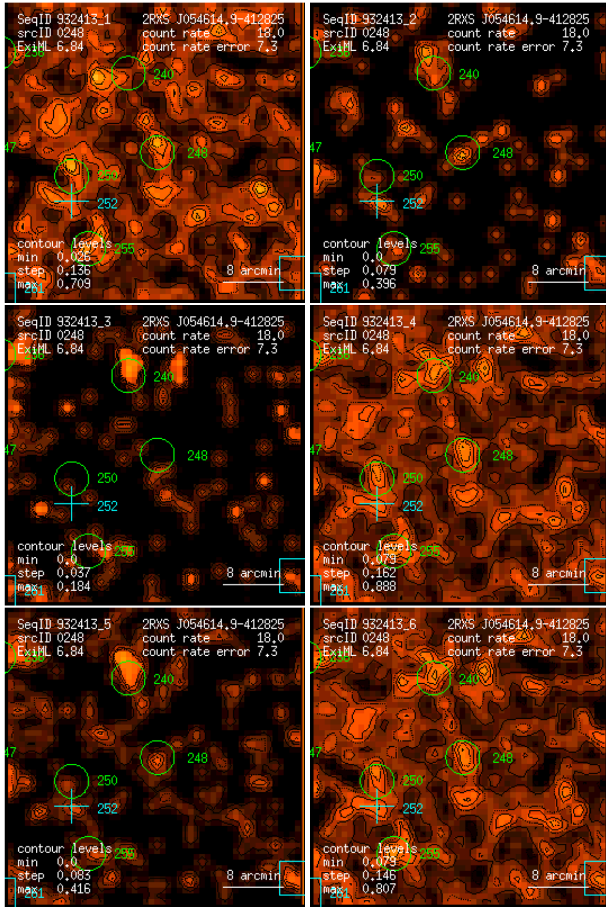
Figure 248: RASS 932413: detection 0248: band rate images, Gaussian filter: (1) PSPC channels 11 – 41, (2) 52 – 90, (3) 91 – 201, (4) 11 – 235, (5) 52 – 201, (6) 11 – 201. Broad band rates in counts/ks. Band rate contour levels in counts/ks/arcmin 2 .
