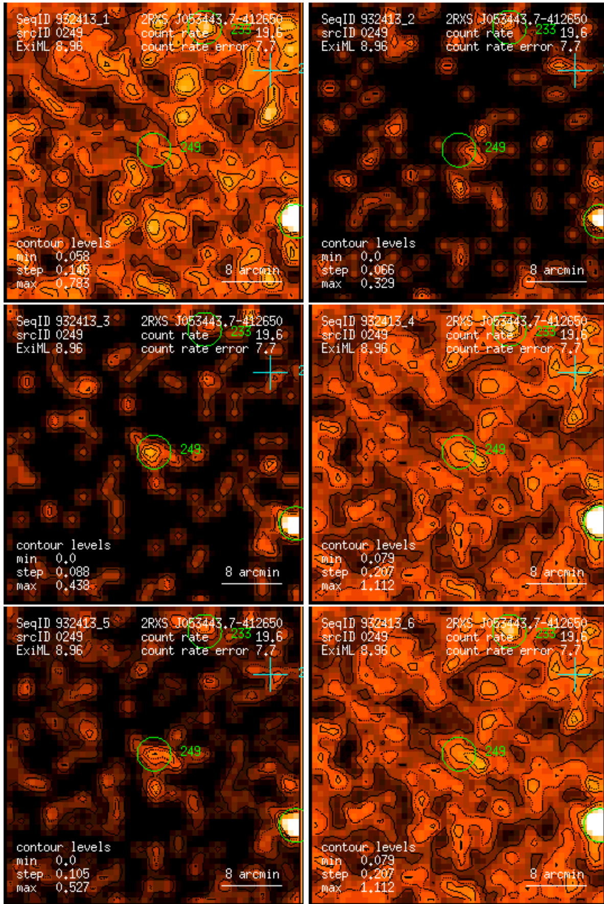
Figure 249: RASS 932413: detection 0249: band rate images, Gaussian filter: (1) PSPC channels 11 – 41, (2) 52 – 90, (3) 91 – 201, (4) 11 – 235, (5) 52 – 201, (6) 11 – 201. Broad band rates in counts/ks. Band rate contour levels in counts/ks/arcmin 2 .
