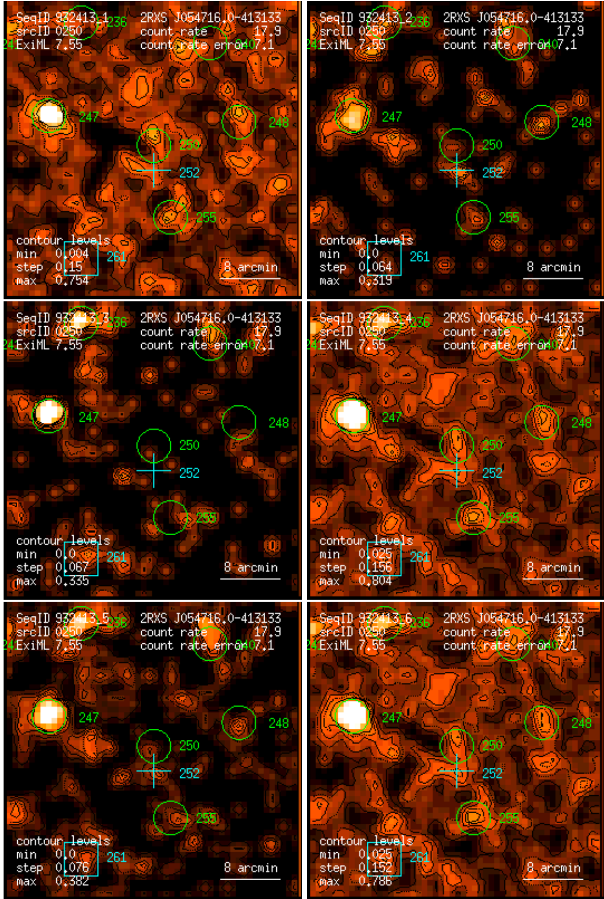
Figure 250: RASS 932413: detection 0250: band rate images, Gaussian filter: (1) PSPC channels 11 – 41, (2) 52 – 90, (3) 91 – 201, (4) 11 – 235, (5) 52 – 201, (6) 11 – 201. Broad band rates in counts/ks. Band rate contour levels in counts/ks/arcmin 2 .
