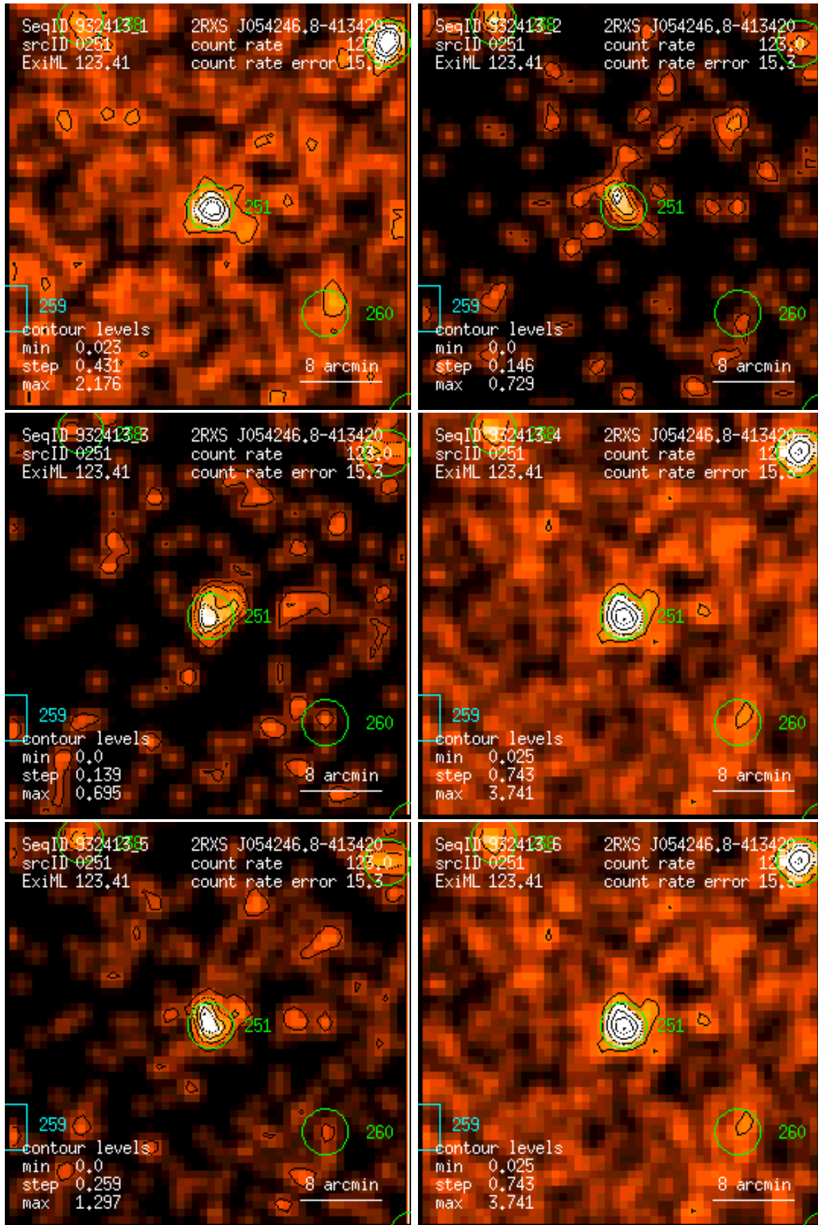
Figure 251: RASS 932413: detection 0251: band rate images, Gaussian filter: (1) PSPC channels 11 – 41, (2) 52 – 90, (3) 91 – 201, (4) 11 – 235, (5) 52 – 201, (6) 11 – 201. Broad band rates in counts/ks. Band rate contour levels in counts/ks/arcmin 2 .
