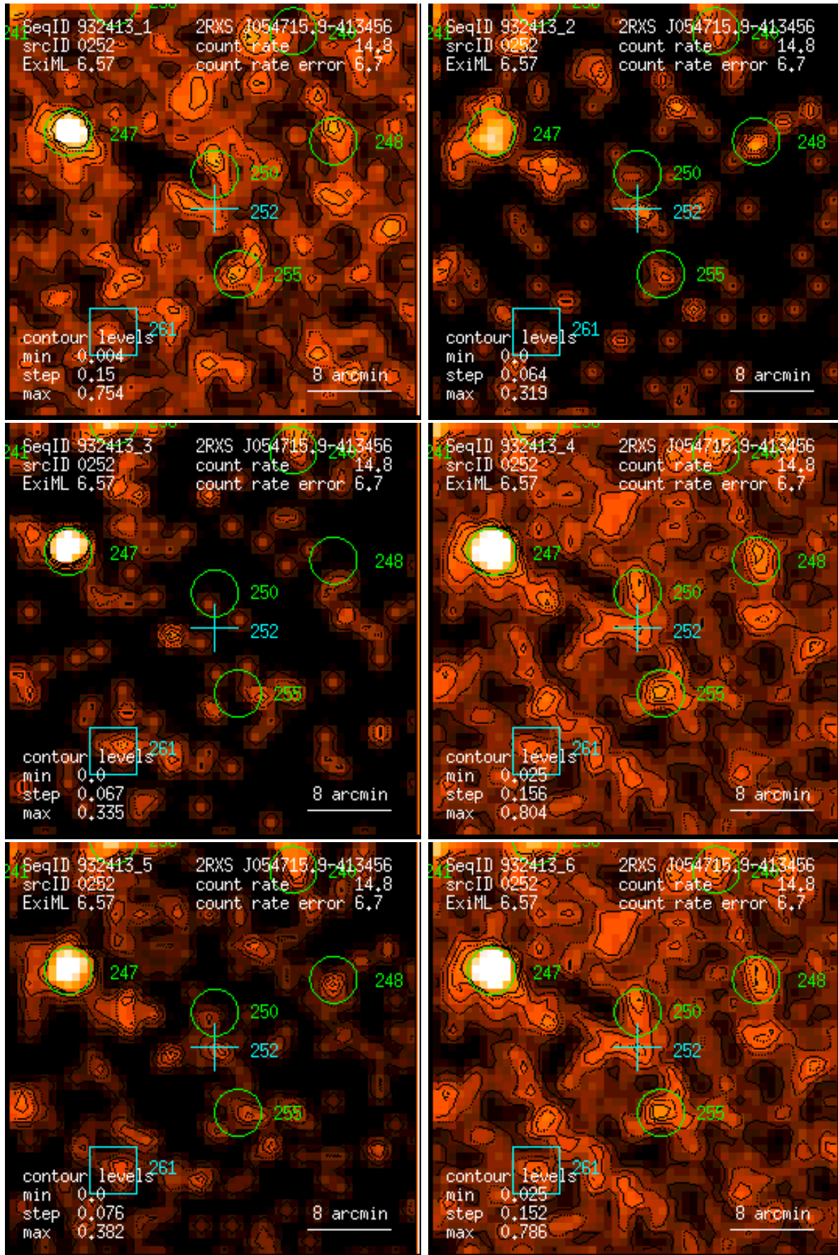
Figure 252: RASS 932413: detection 0252: band rate images, Gaussian filter: (1) PSPC channels 11 – 41, (2) 52 – 90, (3) 91 – 201, (4) 11 – 235, (5) 52 – 201, (6) 11 – 201. Broad band rates in counts/ks. Band rate contour levels in counts/ks/arcmin 2 .
