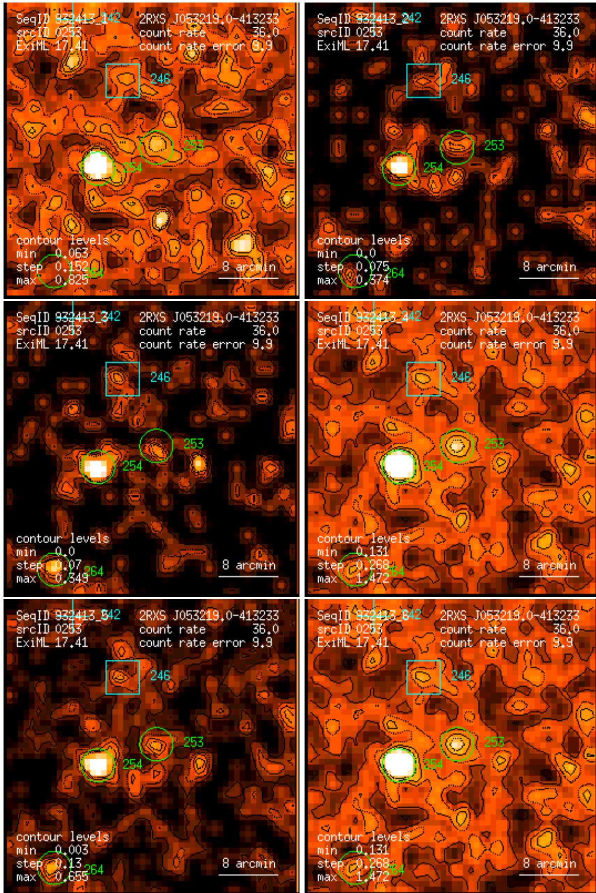
Figure 253: RASS 932413: detection 0253: band rate images, Gaussian filter: (1) PSPC channels 11 – 41, (2) 52 – 90, (3) 91 – 201, (4) 11 – 235, (5) 52 – 201, (6) 11 – 201. Broad band rates in counts/ks. Band rate contour levels in counts/ks/arcmin 2 .
