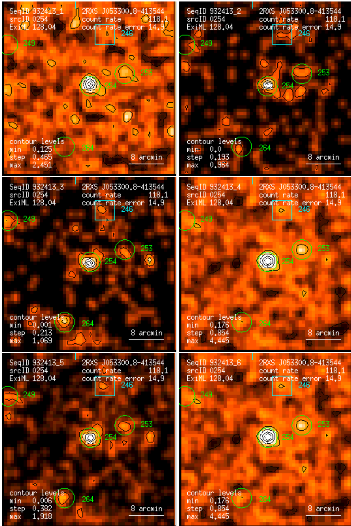
Figure 254: RASS 932413: detection 0254: band rate images, Gaussian filter: (1) PSPC channels 11 – 41, (2) 52 – 90, (3) 91 – 201, (4) 11 – 235, (5) 52 – 201, (6) 11 – 201. Broad band rates in counts/ks. Band rate contour levels in counts/ks/arcmin 2 .
