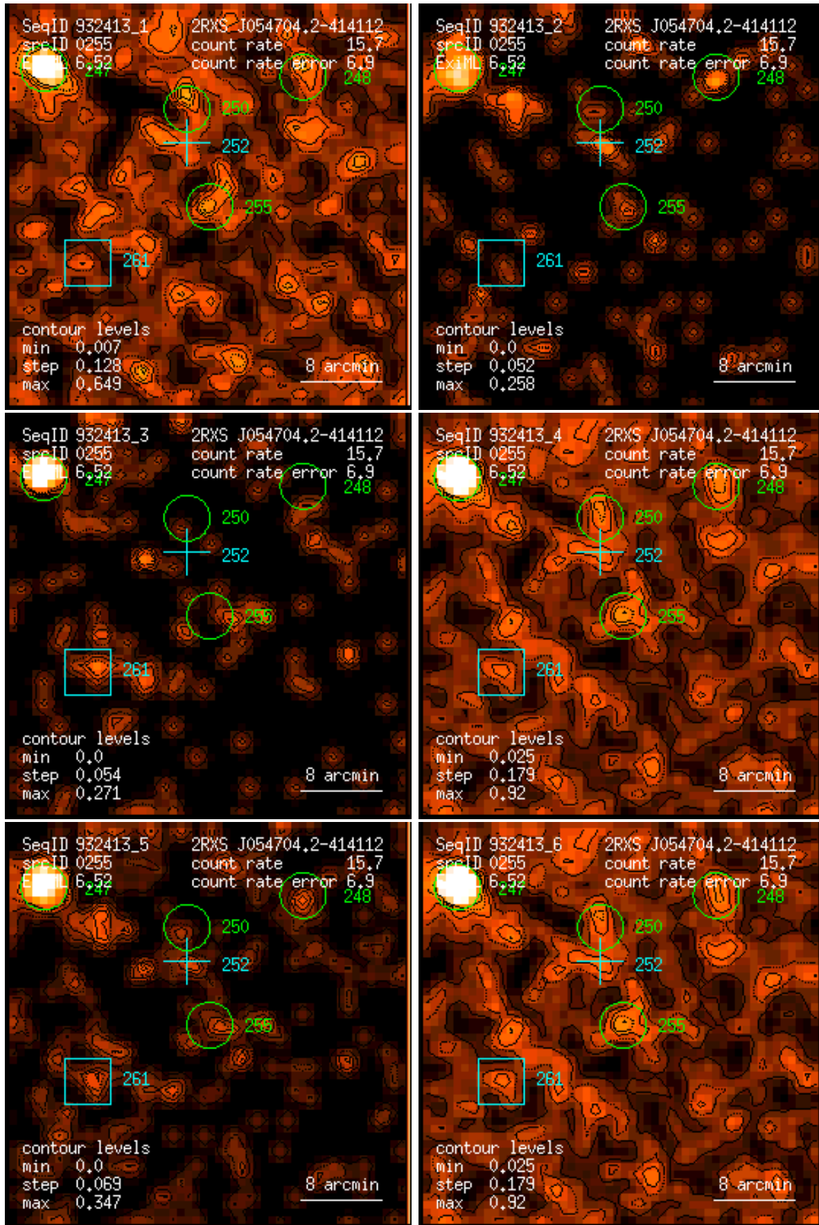
Figure 255: RASS 932413: detection 0255: band rate images, Gaussian filter: (1) PSPC channels 11 – 41, (2) 52 – 90, (3) 91 – 201, (4) 11 – 235, (5) 52 – 201, (6) 11 – 201. Broad band rates in counts/ks. Band rate contour levels in counts/ks/arcmin 2 .
