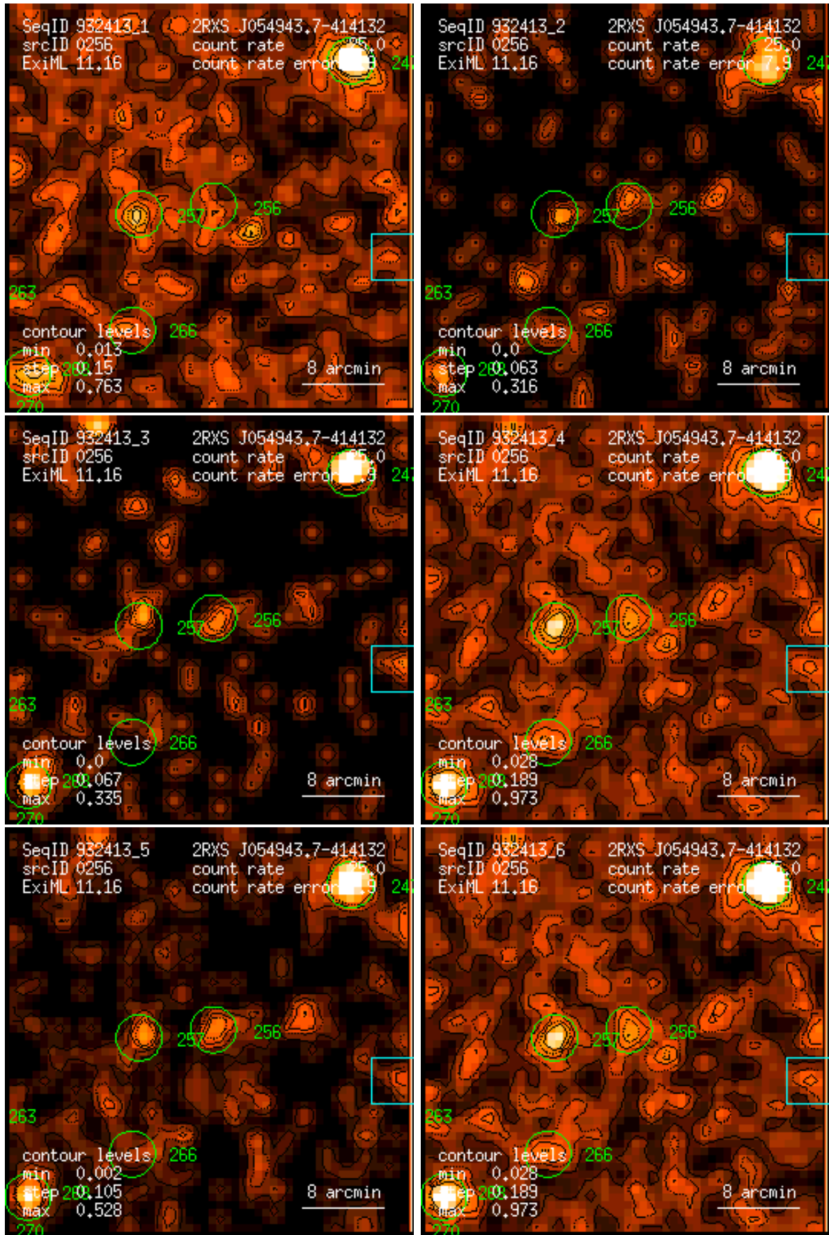
Figure 256: RASS 932413: detection 0256: band rate images, Gaussian filter: (1) PSPC channels 11 – 41, (2) 52 – 90, (3) 91 – 201, (4) 11 – 235, (5) 52 – 201, (6) 11 – 201. Broad band rates in counts/ks. Band rate contour levels in counts/ks/arcmin 2 .
