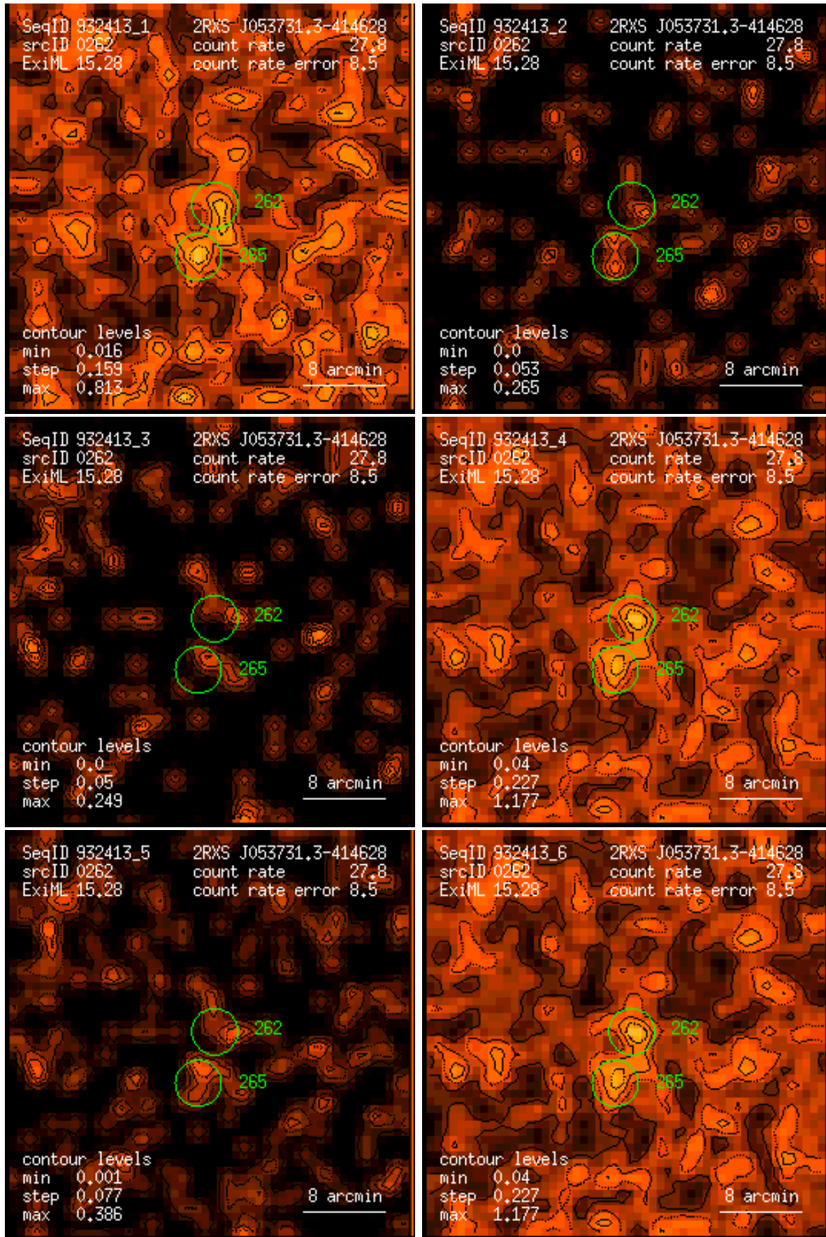
Figure 262: RASS 932413: detection 0262: band rate images, Gaussian filter: (1) PSPC channels 11 – 41, (2) 52 – 90, (3) 91 – 201, (4) 11 – 235, (5) 52 – 201, (6) 11 – 201. Broad band rates in counts/ks. Band rate contour levels in counts/ks/arcmin 2 .
