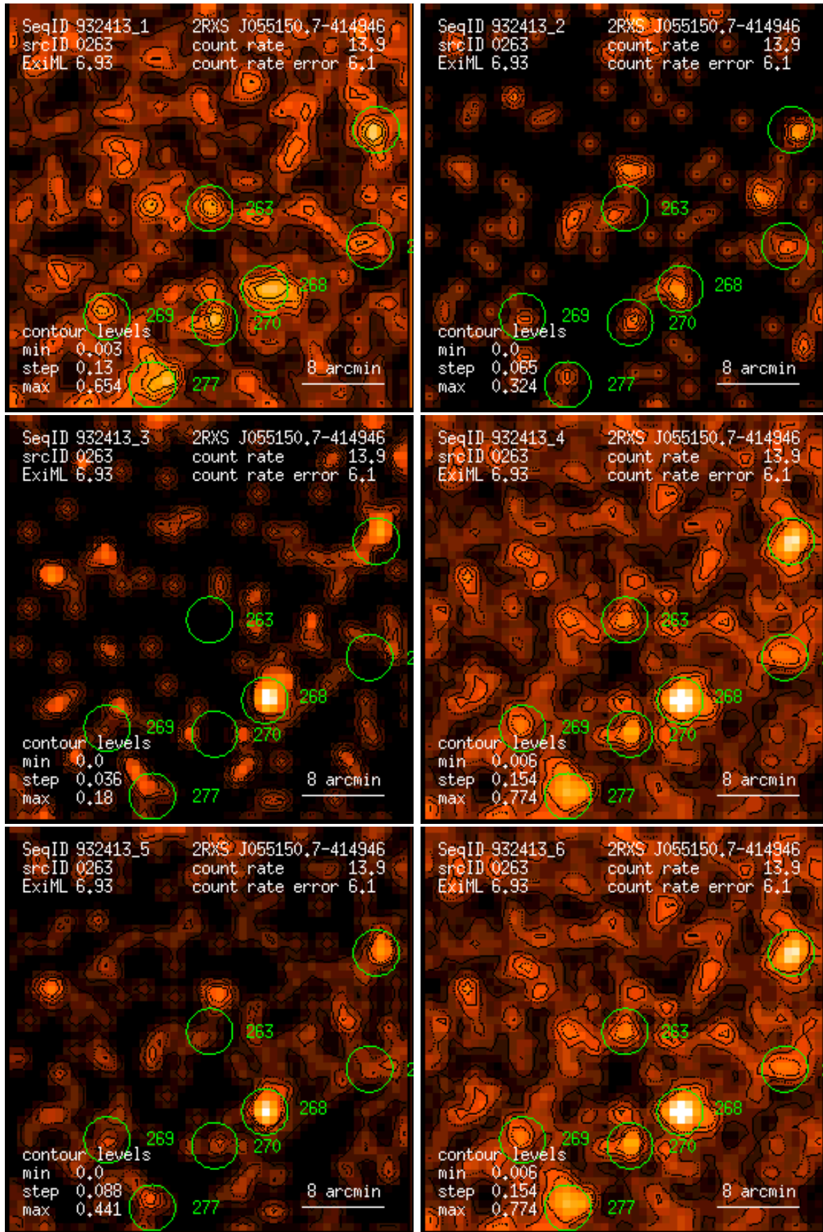
Figure 263: RASS 932413: detection 0263: band rate images, Gaussian filter: (1) PSPC channels 11 – 41, (2) 52 – 90, (3) 91 – 201, (4) 11 – 235, (5) 52 – 201, (6) 11 – 201. Broad band rates in counts/ks. Band rate contour levels in counts/ks/arcmin 2 .
