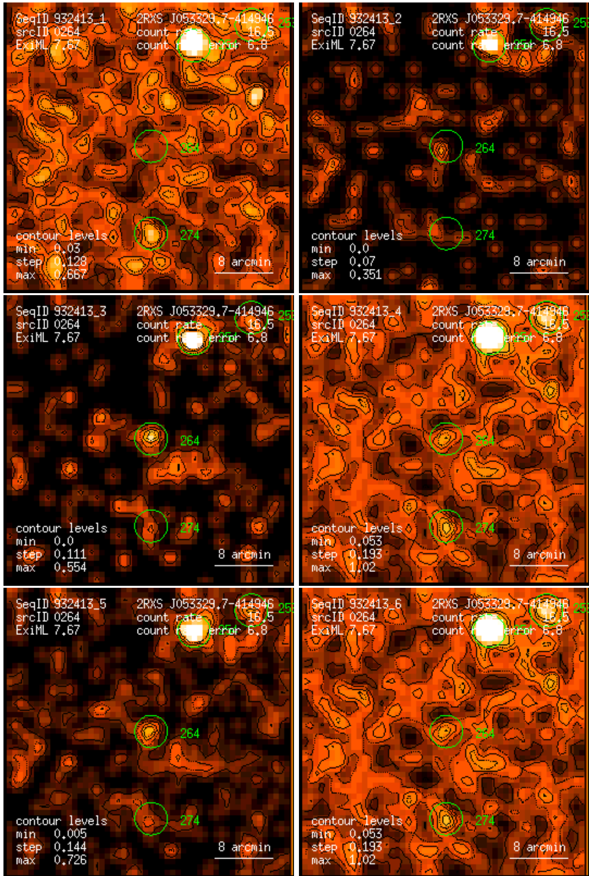
Figure 264: RASS 932413: detection 0264: band rate images, Gaussian filter: (1) PSPC channels 11 – 41, (2) 52 – 90, (3) 91 – 201, (4) 11 – 235, (5) 52 – 201, (6) 11 – 201. Broad band rates in counts/ks. Band rate contour levels in counts/ks/arcmin 2 .
