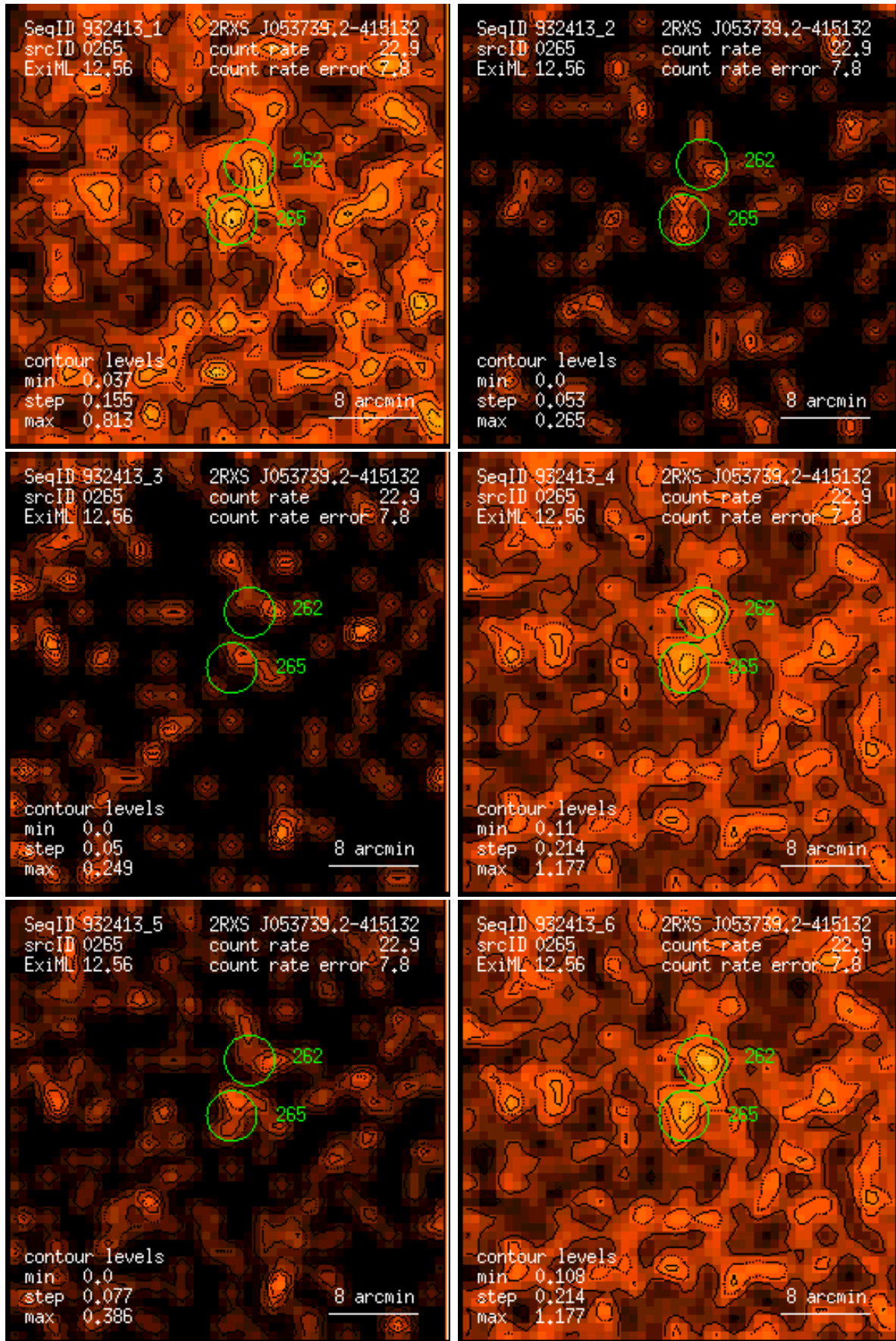
Figure 265: RASS 932413: detection 0265: band rate images, Gaussian filter: (1) PSPC channels 11 – 41, (2) 52 – 90, (3) 91 – 201, (4) 11 – 235, (5) 52 – 201, (6) 11 – 201. Broad band rates in counts/ks. Band rate contour levels in counts/ks/arcmin 2 .
